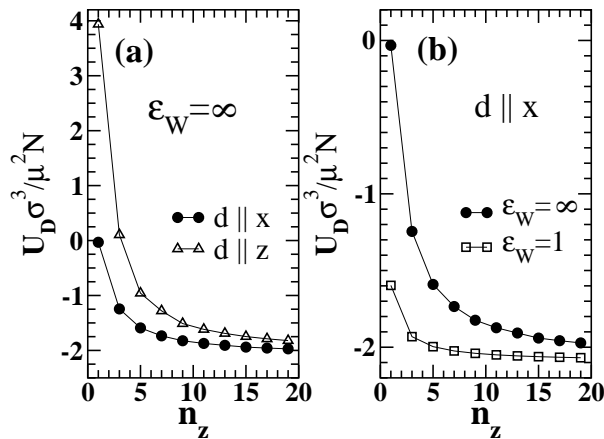
FIG. 11: Dimensionless energy per particle for dipolar crystalline (fcc) slabs with perfect orientational order. Part (a) refers to systems between metallic walls and \hat{\mathbf{d}} \parallel \hat{\mathbf{x}} or \hat{\mathbf{d}} \parallel \hat{\mathbf{z}} . Part (b) compares for the case \hat{\mathbf{d}} \parallel \hat{\mathbf{x}} the energies of systems between metallic and insulating walls [27].
