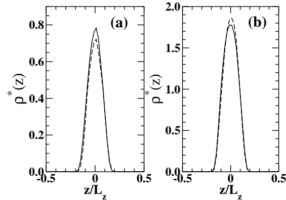
FIG. 7: Local densities at L_z^* = 2.20 and two different parallel pressures P_{\parallel}^* = 0.005 (a) and P_{\parallel}^* = 2.0 (b). The solid and dashed lines indicate results for conducting and insulating walls, respectively.
