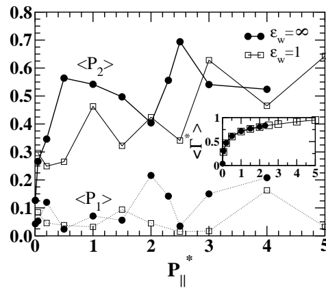
FIG. 8: Order parameters versus parallel pressure P_{\parallel}^* at L_z^* = 2.20 . The solid and open symbols indicate results for conducting and insulating walls, respectively.
