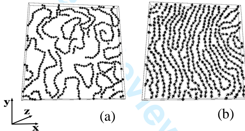
FIG. 9: Snapshots of the system at L_z^* = 2.20 (quasi-monolayer) and \epsilon_w = \infty for two different parallel pressures P_{\parallel}^* = 0.05 (a) and P_{\parallel}^* = 1.0 (b).
