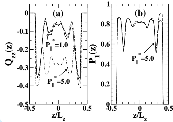
FIG. 6: (a) The local order parameter Q_{zz}(z) at P_{\parallel}^* = 1.0 and P_{\parallel}^* = 5.0 . (b) The local polarization at P_{\parallel}^* = 5.0 . Results for conducting and insulating walls are indicated by solid and dashed lines, respectively.
