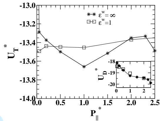
FIG. 10: Energies versus parallel pressure P_{\parallel}^* at L_z^* = 2.20 . The solid and open symbols indicate results for conducting and insulating walls, respectively.
