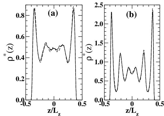
FIG. 5: Local number density at (a) P_{\parallel}^* = 1 (isotropic phase) and (b) P_{\parallel}^* = 5 (ferroelectric phase). Results for conducting and insulating walls are indicated by solid and dashed lines, respectively.
