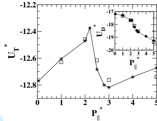
FIG. 4: Energies versus parallel pressure P_{\parallel}^* at L_z^* = 7.0 . The solid and open symbols indicate results for conducting and insulating walls [27], respectively.
