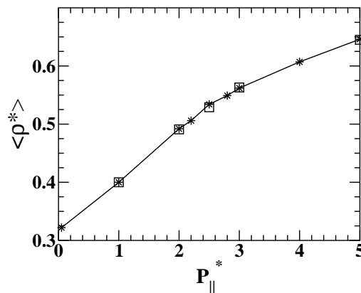
FIG. 3: Density versus parallel pressure P_{\parallel}^* at L_z^* = 7.0 . The solid and open symbols indicate results for conducting and insulating walls, respectively.
