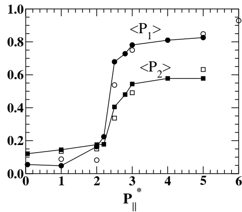
FIG. 2: Order parameters \langle P_1 \rangle and \langle P_2 \rangle versus parallel pressure P_{\parallel}^* at wall separation L_z^* = 7.0 ( T^* = 1.35 and m^* = 3.0 ). The solid and open symbols indicate MC results for conducting and insulating walls [27], respectively.
