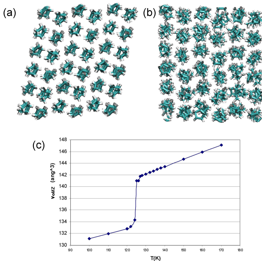
Snapshots of Molecular Dynamics simulations of cyclopentane. (a) monoclinic ordered phase III at 100 K viewed along b (b) hexagonal disordered phase I at 170 K, viewed along b , and (c) a plot of the variation in cell volume with temperature.
