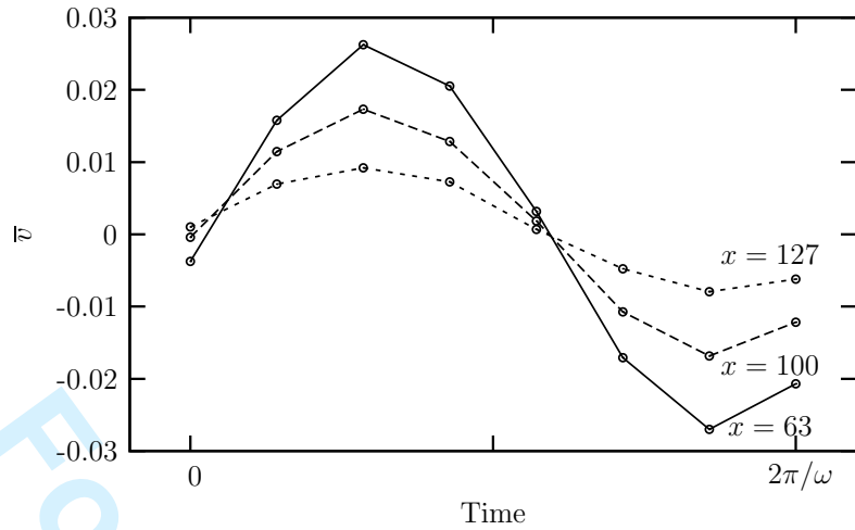
Figure 7: Averaged stream velocities, \bar{v} , in the y -direction in the main channel and for different values of x as a function of time for \omega = 0.053 . The lines are a guide to the eye.
