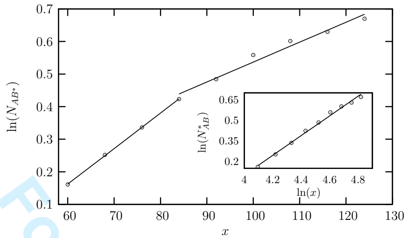
Figure 3: \ln(N_{AB}^*) as a function of x for \omega = 0.053 . Lines are the best fits to the data. Superimposed figure shows \ln(N_{AB}^*) as a function of \ln(x) when the mixing device is switched off. The slope is 0.75.
