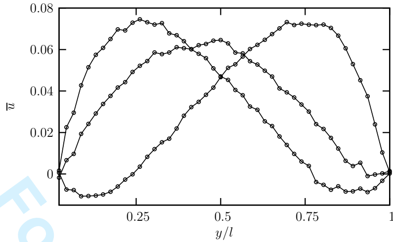
Figure 6: Velocity profiles for three different times just downstream from the mixing intersection and for \omega = 0.053 . The lines are a guide to the eye.
