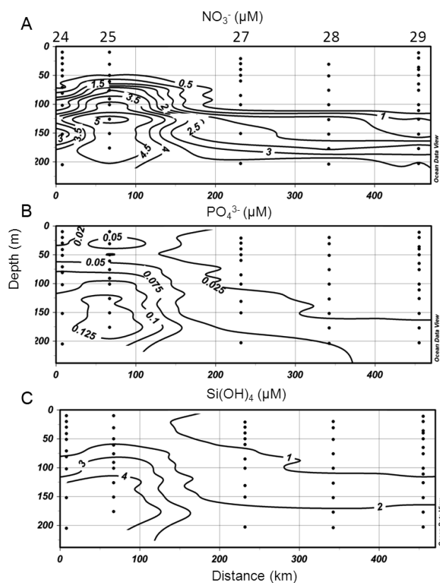
Fig. 7. Vertical distribution of (a) nitrate ( \text{NO}_3^- ), (b) phosphate ( \text{PO}_4^{3-} ) and (c) silicate ( \text{Si}(\text{OH})_4 ) down to 200 m along the north-south transect defined by stations 24 to 29.
