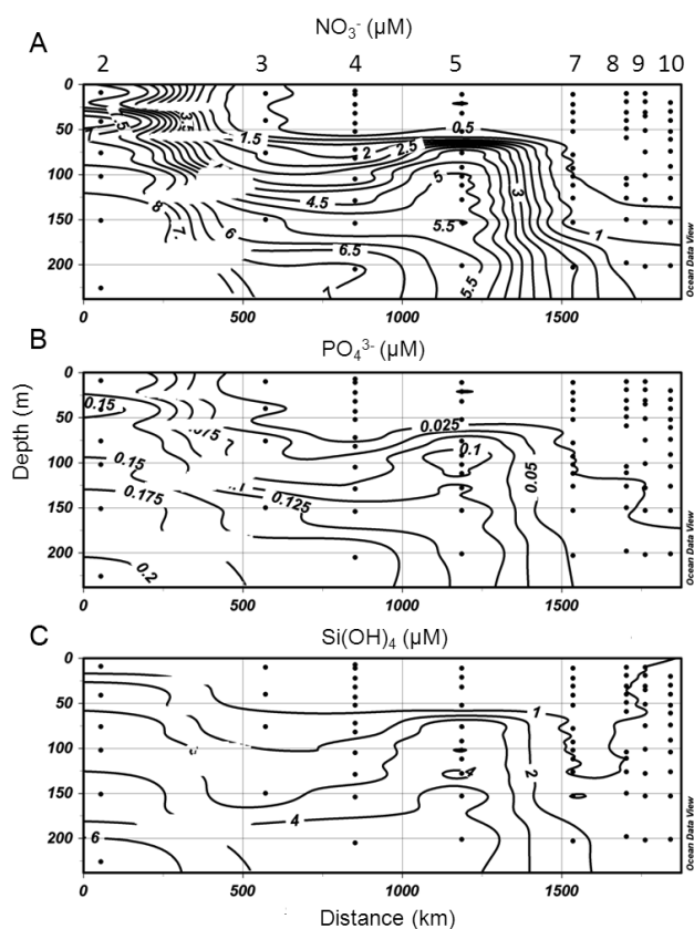
Fig. 11. Vertical distribution of (A) nitrate ( \text{NO}_3^- ), (B) phosphate ( \text{PO}_4^{3-} ) and (C) Silicate \text{Si(OH)}_4 down to 200 m across the western Mediterranean Sea and the western part of the Ionian basin.
