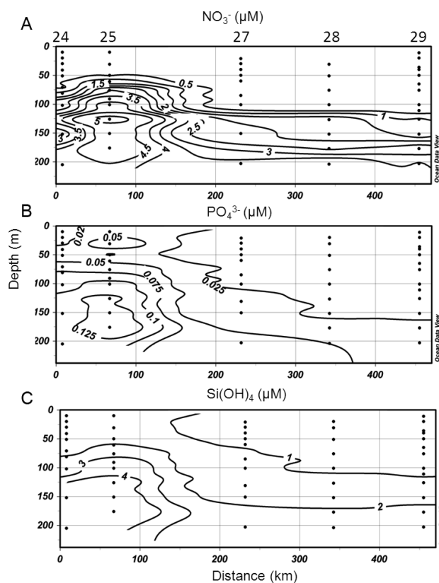
Fig. 7. Vertical distribution of (a) nitrate ( \text{NO}_3^- ), (b) phosphate ( \text{PO}_4^{3-} ) and (c) silicate ( \text{Si(OH)}_4 ) down to 200 m along the north-south transect defined by stations 24 to 29.
