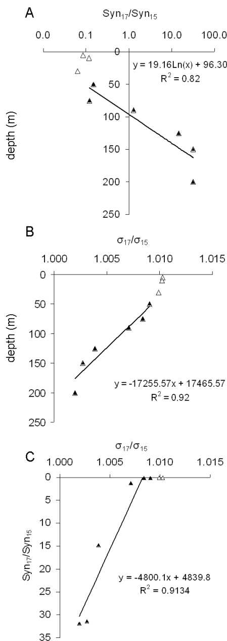
Fig. 5. Relationships between vertical distributions of Synechococcus abundance and density inside (station 17) and outside (station 15) the south Adriatic gyre. (A) Depth dependence of the abundance ratio \text{Syn}_{17}/\text{Syn}_{15} . (B) Depth dependence of the density ratio \sigma_{17}/\sigma_{15} . (C) Relationship between Synechococcus abundance ratio \text{Syn}_{17}/\text{Syn}_{15} and density ratio \sigma_{17}/\sigma_{15} . Data belonging to the upper 50 m (empty triangles) were excluded from the relationships (filled triangles).
