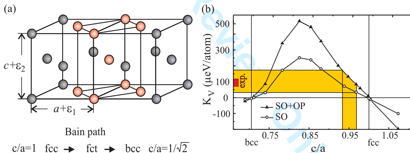
51 Figure 1. (color online) a) Transformation of an fcc into a bcc structure via the Bain path. b) ab initio calculation of K_V for an 52 infinite-sized Ni single crystal, using spin-orbit coupling (open circles), only, and adding orbital polarization (full triangles), also. [9].
