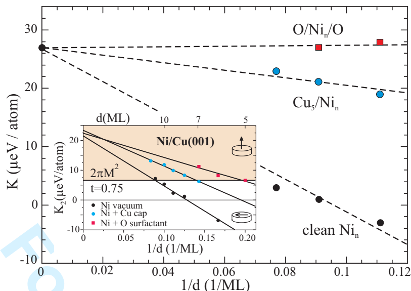
Figure 5. (color online) Calculated MAE for clean Ni films, Cu 5 /Ni n /Cu superlattices, and Ni films with a c(2x2) oxygen adlayer [19]. The inset shows the corresponding experiments. For details see text.
