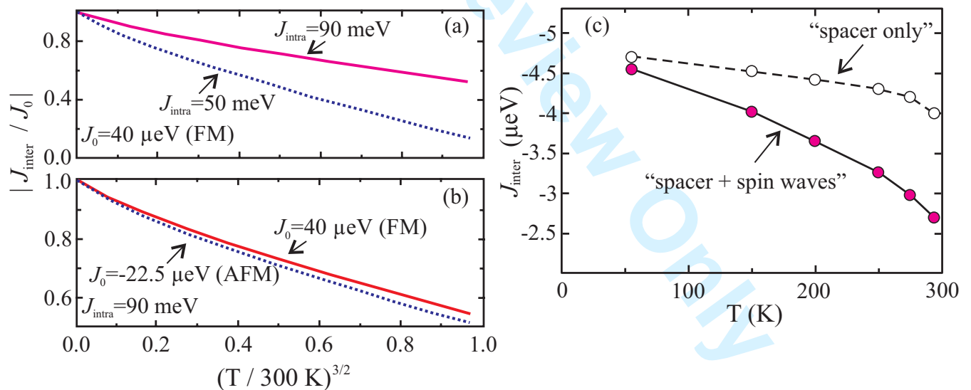
Figure 8. (color online) J_{\text{inter}}/J_0 vs. T^{3/2} for a fixed J_0 in a) and for fixed J_{\text{intra}} in b), from [26]. c) shows J_{\text{inter}} as function of T, calculated with and without spin wave excitation [27].
