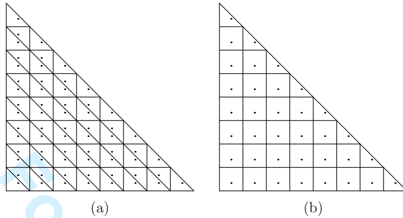
Figure 2: The two alternative discretizations of the state space of Dirichlet distribution.
