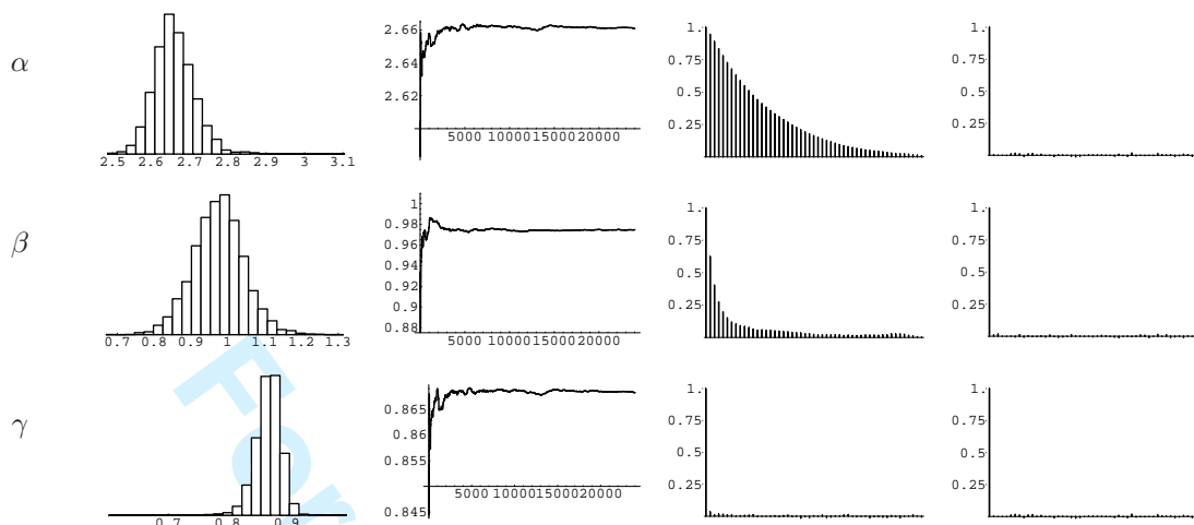
Figure 4: Histograms, convergence of the weighted means \hat{\alpha}_n^{IS} , \hat{\beta}_n^{IS} and \hat{\gamma}_n^{IS} and autocorrelations of the unweighted samples (\alpha_i)_{1 \leq i \leq 20000} , (\beta_i)_{1 \leq i \leq 20000} and (\gamma_i)_{1 \leq i \leq 20000} and of the weighted samples (\alpha_i, w(\theta_i))_{1 \leq i \leq 20000} , (\beta_i, w(\theta_i))_{1 \leq i \leq 20000} and (\gamma_i, w(\theta_i))_{1 \leq i \leq 20000} with m = 5 after a 5000 burn-in period for the dugongs dataset.
