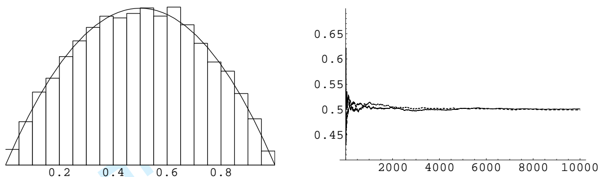
Figure 1: Histogram of the weighted sample (x_i, w(x_i))_{1 \leq i \leq 10000} and convergence of the weighted mean \hat{x}_n^{IS} = \sum w(x_i)x_i / \sum w(x_i) for m = 10 (solid line) and of the sample mean of an iid sample from the target distribution (dashed line).
