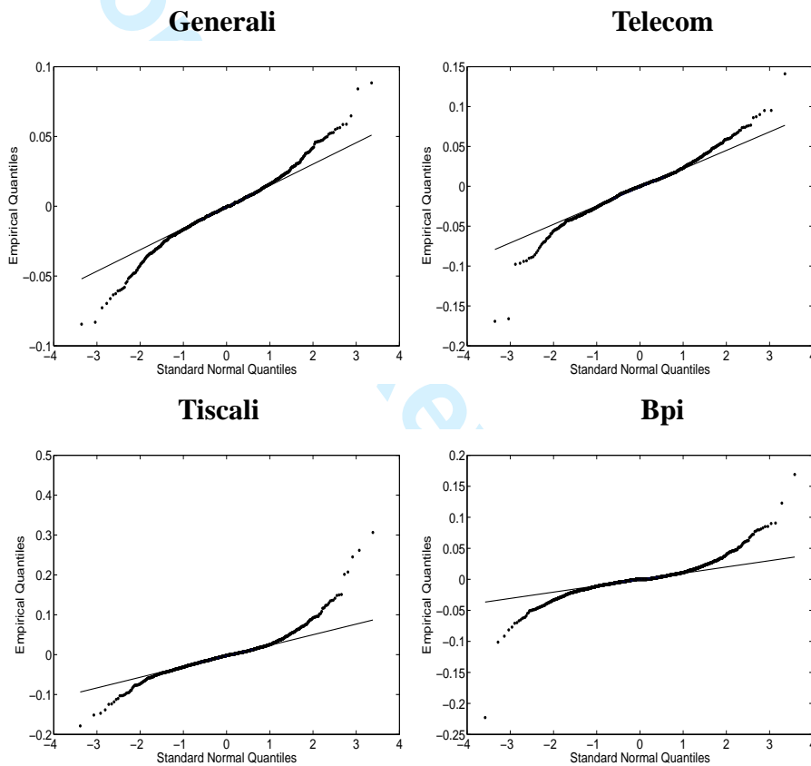
Figure 2: Normal QQ-plot for daily returns.
