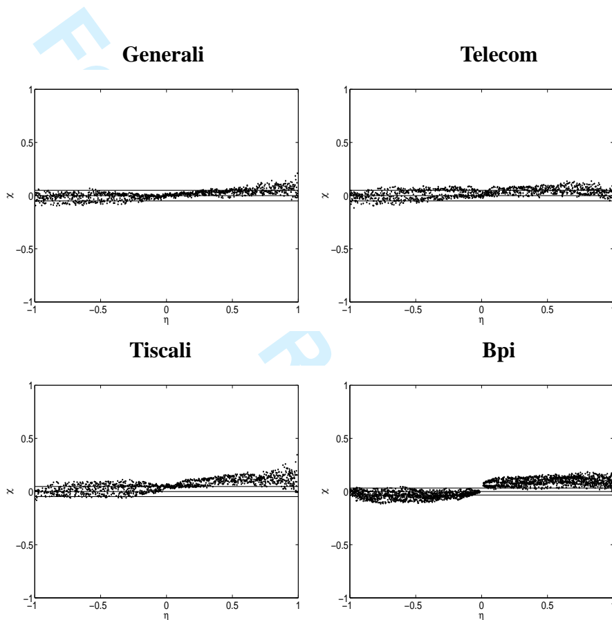
Figure 5: Chi-plot for daily returns.
