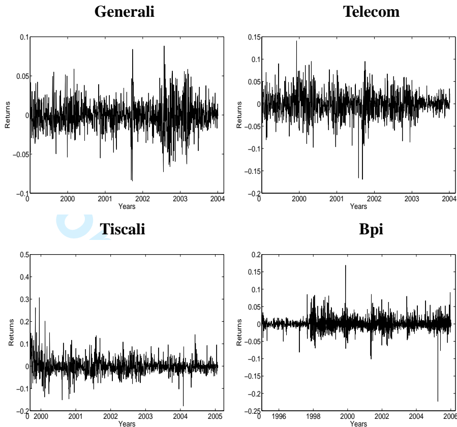
Figure 4: Daily returns and volatility cluster phenomenon.
