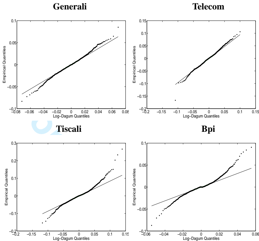
Figure 3: Log-Dagum QQ-plot for daily returns.
