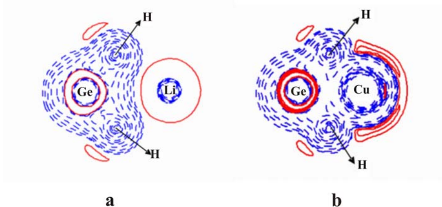
Figure 18. Energy density contour maps for the germane- \text{Li}^+ (a) and germane- \text{Cu}^+ (b) complexes. The energy density has been plotted in a plane containing the silicon atom, as well as the two hydrogen atoms interacting with the metal ion.
