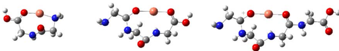
Figure 12. B3LYP optimized geometries for the global minima of the diglycine-, triglycine- and tetraglycine- \text{Cu}^+ potential energy surfaces taken from ref. 31
