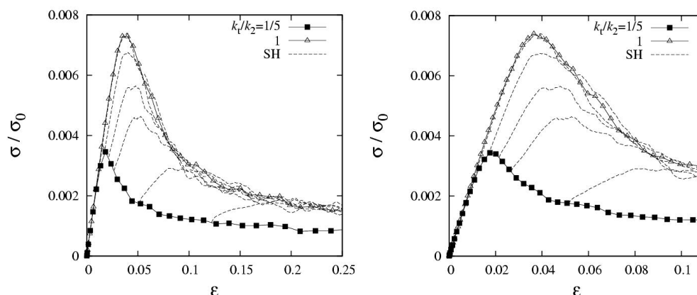
Fig. 4 (Left) Axial stress versus axial strain during uniaxial compression. Lines with solid squares and open triangles represent the damage responses of the relatively weak ( k_t/k_2=1/5 ) and strong ( k_t/k_2=1 ) samples, respectively, as taken from Fig. 3. The dashed lines reflect the responses after the initiation of self-healing (which occurs by increasing the particle contact adhesion to k_t/k_2=1 ) at various deformation levels. (Right) Magnification of the responses plotted in the left figure; the initiation of self-healing occurs at axial strains \epsilon \approx 0.016, 0.019, 0.022, 0.026, 0.045, and 0.12 .
