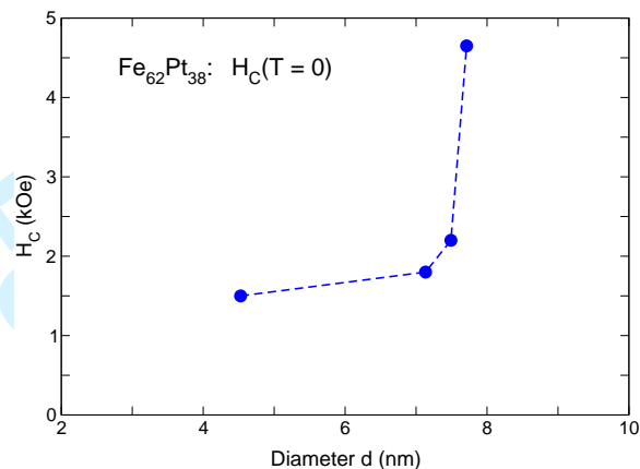
9 10 11 12 13 14 15 16 17 18 19 20 21 22 23 24 25 26 27 28 29 30 31 32 33 34 35 36 37 38 39 40 41 42 43 44 45 46 47 48 49 50 51 52 53 54 55 56 57 58 59 60 Figure 5. Coercivity fields as a function of the size of the Fe_{62}Pt_{38} clusters. The data have been extrapolated to zero temperature from the room temperature measurements of the hysteresis curves. Figure adapted from [42].
