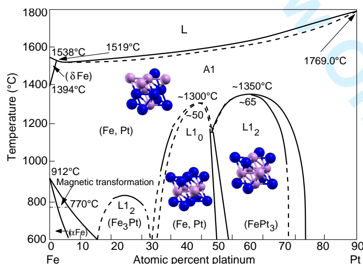
Figure 6. Equilibrium phase diagram and crystallographic structures of FePt with the L_{10} structure around 50 at.% Fe. The magnetic properties of thin films, nanocrystalline materials and nanoparticles differ depending on the approach used to achieve the L_{10} phase. Figure adapted from [59, 62].
