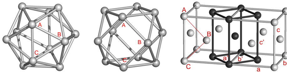
Figure 1. Left and center: Icosahedron and cuboctahedron - during the Mackay transformation, the bond \overline{AC} (left) stretches and the two adjacent triangles turn into the same plane. The capital letters refer to the same atomic sites in each structure. Right: Face-centered cubic lattice with inscribed body-centered tetragonal Bain cell. The Bain transformation is controlled by variation of c with respect to a and b . Figure adapted from [13], copyright (2007) by the American Physical Society.
