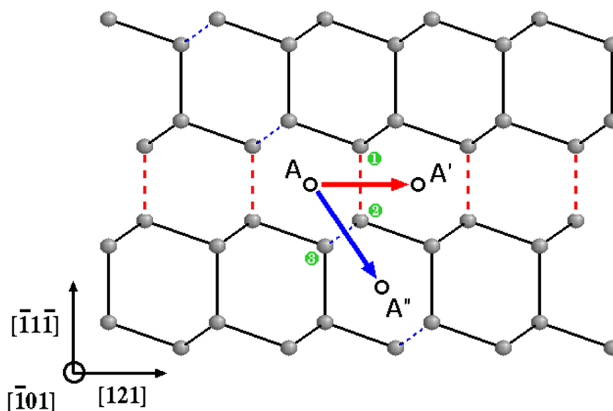
Figure 2. (color online) Ball-and-stick representation of the zinc-blende structure ( (\bar{1}01) plane). The path D' ( D'' ) is defined by a dislocation displacement from A to A' ( A to A'' ). Dashed lines show bonds linking atoms used for calculating the disregistry due to the dislocation core. In particular, atoms located in dislocation cores for saddle configurations are marked by numbers (1 and 2 for D' , and 2 and 3 for D'' ).
