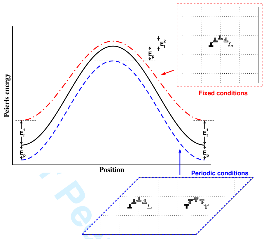
Figure 1. (color online) Effect of boundary conditions on Peierls energy variation as a function of the dislocation core position. For fixed conditions, the interaction between the single dislocation and the surface cluster ranges from E_f^1 to E_f^2 (dash-dotted line). By combining periodic conditions and NEB, and by displacing the dislocations coherently, the interaction E_p between dislocations remains constant (dashed line) and does not affect the deduced Peierls stress and activation energy.
