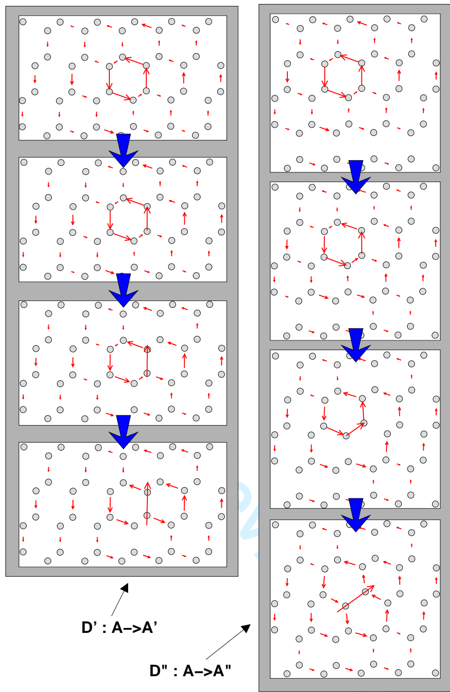
Figure 4. (color online) Differential displacement maps corresponding to screw dislocation displacements along D' (left) and D'' (right), between A and the saddle configurations. The arrows are proportional to the out-of-plane [101] shifts between neighbouring atoms introduced by the dislocation.
