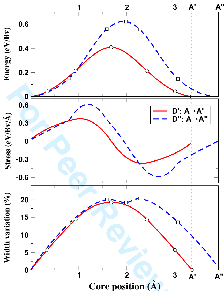
Figure 3. (color online) Energy (in eV/Burgers vector, top graph), stress (derivative of the plotted energy curves, middle graph), and core width variation (bottom graph) as a function of the dislocation core position in the lattice for paths D' (full lines) and D'' (dashed lines).
