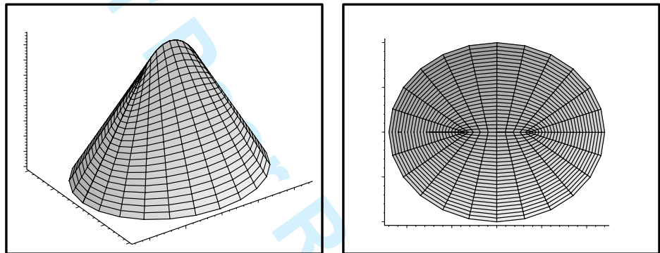
20 21 22 23 24 25 26 27 28 29 30 31 32 33 Figure 1. Side and top views of a portion of a conical constant-angle surface with vertical uniform orientation field 34 \mathbf{m} = \mathbf{m}_0 . The plane curve generating the cone is an ellipse.
