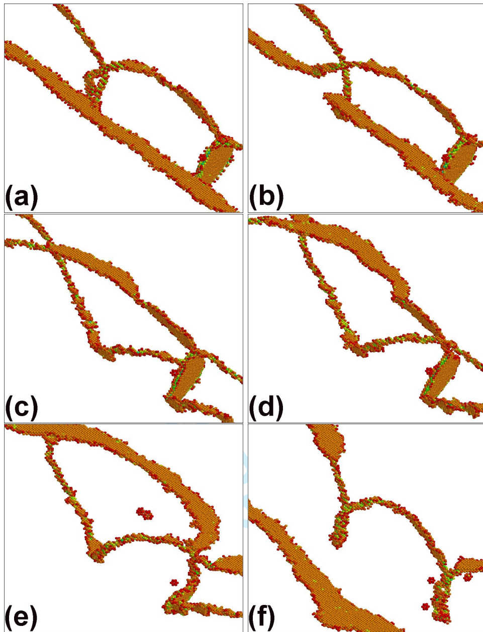
Figure 5. Two screw dislocations in presence of both W^- and W^+ loops ( 2SD, B^-, S^-, P1 and P2 ): snapshots shown at 195 MPa, 140 ps (a), 200 MPa, 145 ps (b), 205 MPa, 155 ps (c), 210 MPa, 165 ps (d), 215 MPa, 163 ps (e), 215 MPa, 193 ps (f).
