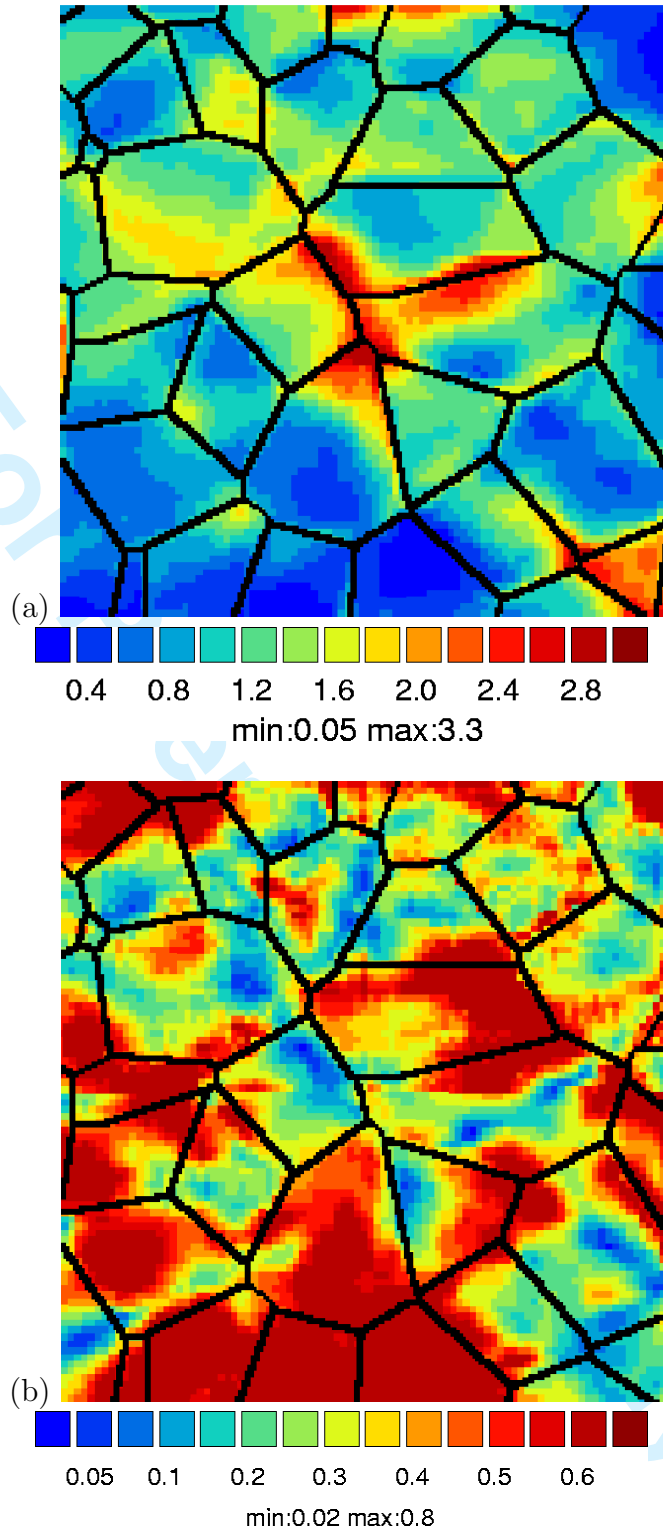
Fig. 7. (a) Ensemble average of the cumulative plastic slip field \bar{\gamma}_{eq}(\underline{x}) / \langle \bar{\gamma}_{eq} \rangle at the constrained free surface of the polycrystalline aggregates in tension. (b) Relative variance D(\gamma_{eq})(\underline{x}) / \bar{\gamma}_{eq}(\underline{x}) of the local plastic slip at the constrained free surface. Tension is applied along vertical direction y . The prescribed overall tensile strain is E_{22} = 0.02 .
