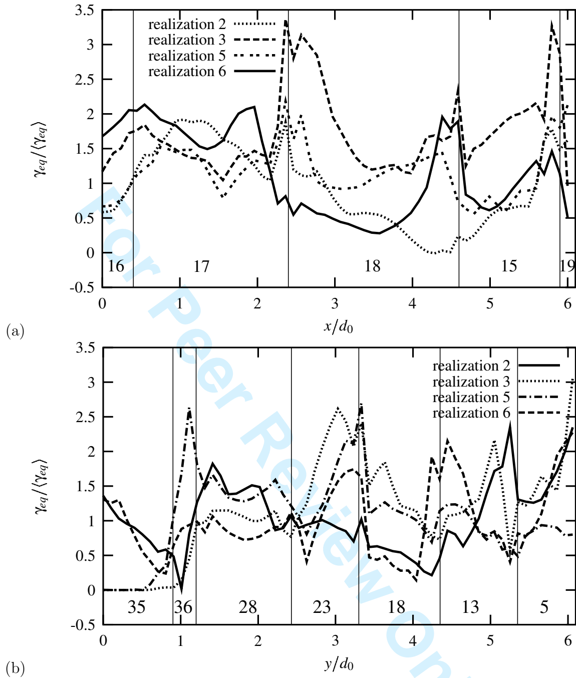
Fig. 5. Cumulative plastic slip profiles along the lines hline (a) and vline (b) of figure 1 for four different realizations of polycrystalline aggregates with a prescribed free surface and subjected to simple tension. The stress distribution is normalized by the global mean stress \langle \gamma_{eq} \rangle over all realizations. The vertical lines indicate the x -position of the intersection between the grain boundaries and the line hline . The labels of the corresponding grains are recalled. The prescribed overall tensile strain is E_{22} = 0.02 .
