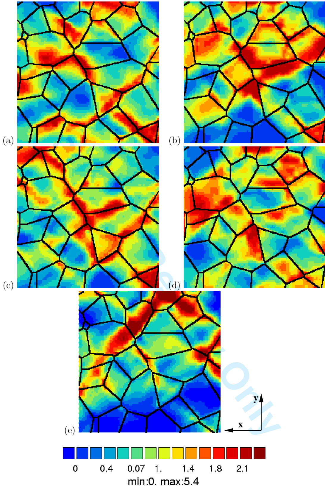
Fig. 4. Cumulative plastic slip distribution \gamma_{eq}(\underline{x}) normalized by the global mean cumulative plastic slip \overline{\langle \gamma_{eq} \rangle} for four different 3D realizations (a) to (d) of the polycrystalline aggregates with a constrained surface geometry. The tensile loading direction y is vertical. The plane of observation is the constrained free surface z = 0 , the geometry of which was given in figure 1. The plastic slip map is also given for the columnar grain microstructure in (e). Grain boundaries are in bold. The prescribed overall tensile strain is E_{22} = 0.02 . The value of \overline{\langle \gamma_{eq} \rangle} was 0.0442.
