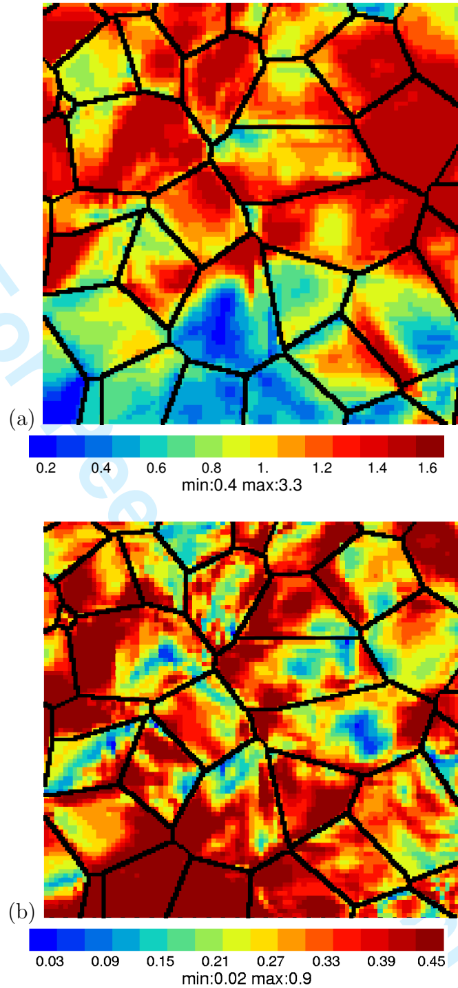
Fig. 10. (a) Ensemble average of the lattice rotation angle field \overline{\phi_c(\mathbf{x})} (in degree) at the constrained free surface of the polycrystalline aggregates in tension. (b) Field of the relative variance D(\phi_c(\mathbf{x})/\overline{\phi_c(\mathbf{x})} of the local lattice rotation at the constrained free surface. Tension is applied in the vertical direction y . The prescribed overall tensile strain is E_{22} = 0.02 .
