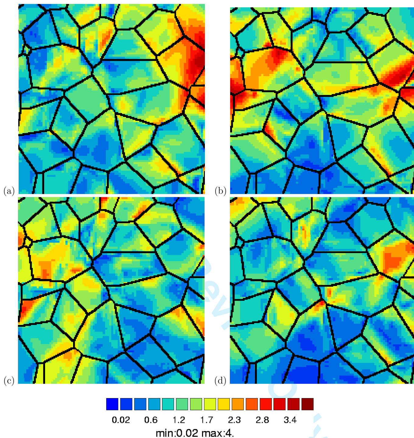
Fig. 9. Lattice rotation maps (in degrees) for four different polycrystalline aggregates with a prescribed free surface geometry. The mapped quantity is the positive part of the lattice rotation angle \phi_c(\underline{x}) . The overall tensile strain is E_{22} = 0.02 . The tensile direction y is vertical. The four realizations (a) to (d) are the same as those presented in figure 4.
