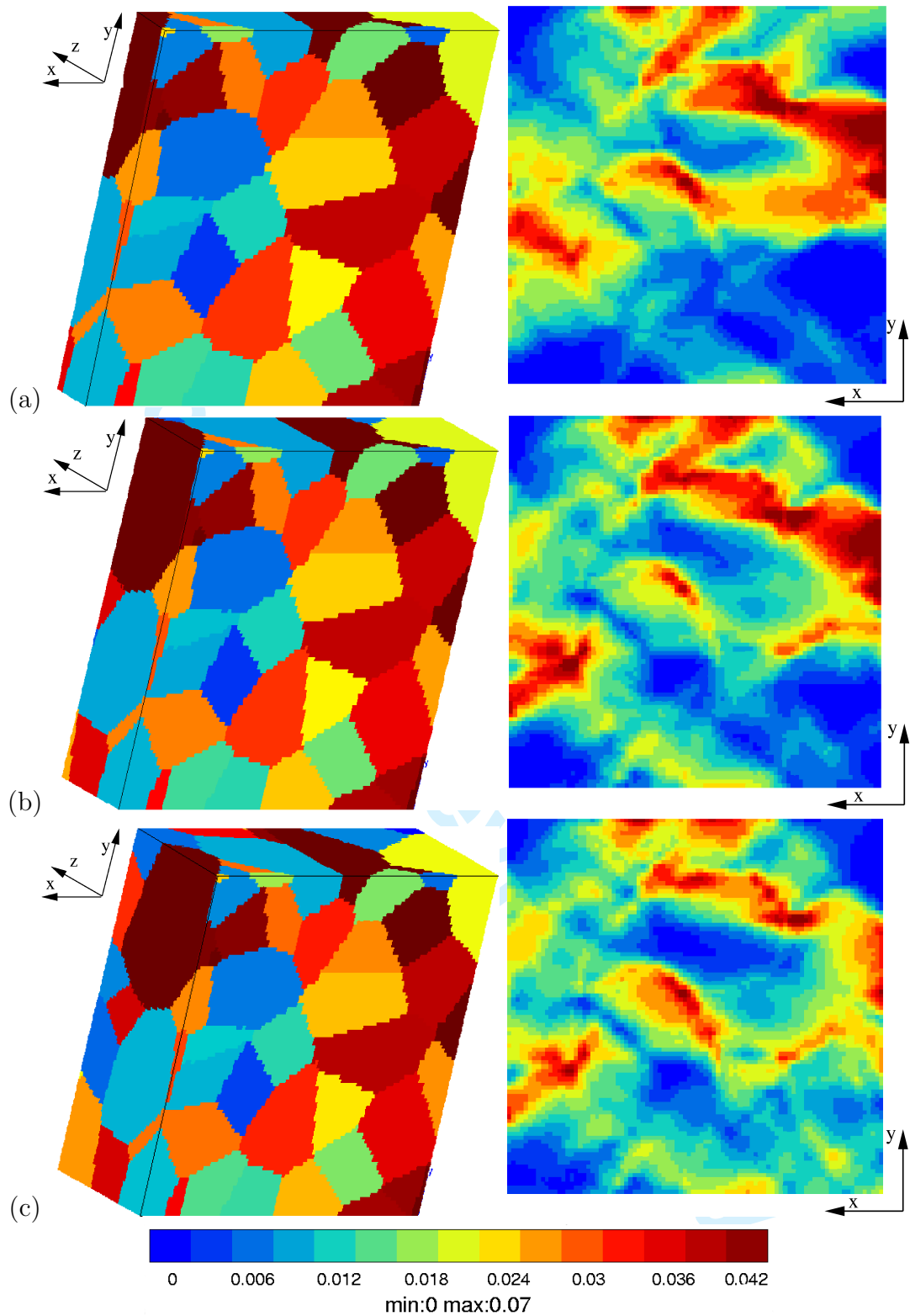
Fig. 2. Influence of the sample thickness on the plastic strain field at the free surface. Three different average numbers of grains within the thickness are considered: (a) 1 grain, (b) 1.5 grain, (c) 2 grains. The cumulative plastic slip \gamma_{eq} fields are given for E_{22} = 0.01 . The three samples are slices with different thicknesses of a large given 3D polycrystalline aggregate containing the constrained free surface of figure 1.
