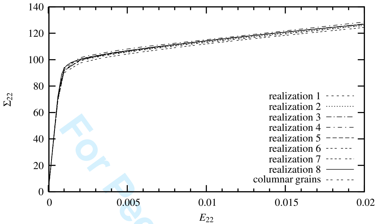
Fig. 3. Overall tensile curves of the 9 polycrystalline aggregates with constrained free surface geometry. For each sample, the mean stress component \Sigma_{22} = \langle \sigma_{22} \rangle is given as a function of the mean strain component E_{22} = \langle \varepsilon_{22} \rangle .
