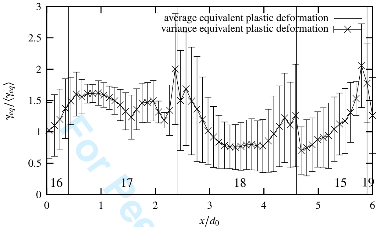
Fig. 8. Ensemble average and variance of the cumulative plastic slip profile along the line hline belonging to the constrained free surface of figure 1. The local value \gamma_{eq}(\underline{x}) is normalized by the mean value of the ensemble average of plastic slip \langle\gamma_{eq}\rangle . The vertical lines indicate the intersection of grain boundaries with line hline . The prescribed overall tensile strain is E_{22} = 0.02 .
