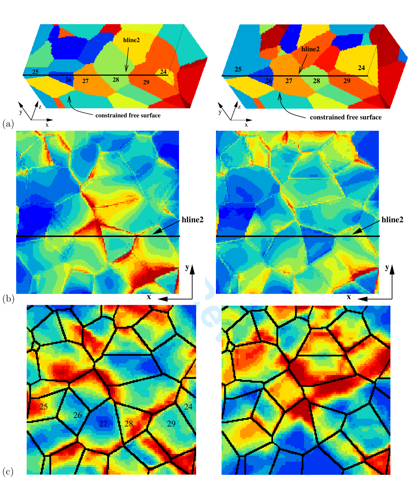
53 Fig. 6. Influence of the 3D grain shape on the stress–strain levels at the constrained free surface. Two 54 realizations of the polycrystalline aggregates with a constrained free surface geometry have been cut 55 along a plane perpendicular to the free surface and containing horizontal line hline2 , see (a). The von Mises 56 equivalent stress fields obtained under the assumption of an elastic local response, are shown in (b). The 57 corresponding results for an elastoplastic local response are shown in (c), the cumulative plastic slip maps 58 (the color scale is the same as in figure 4). 59 60
