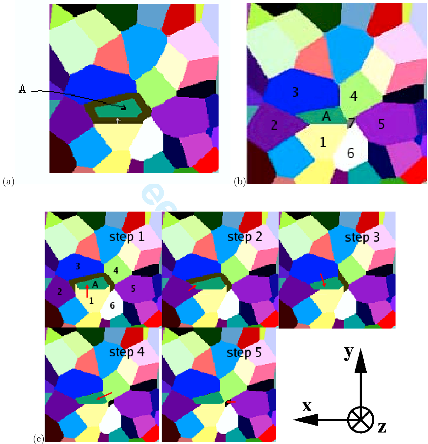
Fig. 2. Erosion of a grain belonging to a given surface and its modification due to the growth of neighbouring grains: (a) the considered grain A is eroded, (b) final environment of grain A, (c) the five growth steps of the grains surrounding grain A necessary to get picture (b). The i^{th} step of figure (c) corresponds to the normal growth of one grain boundary of neighbour grain i , as indicated by the red arrow.
