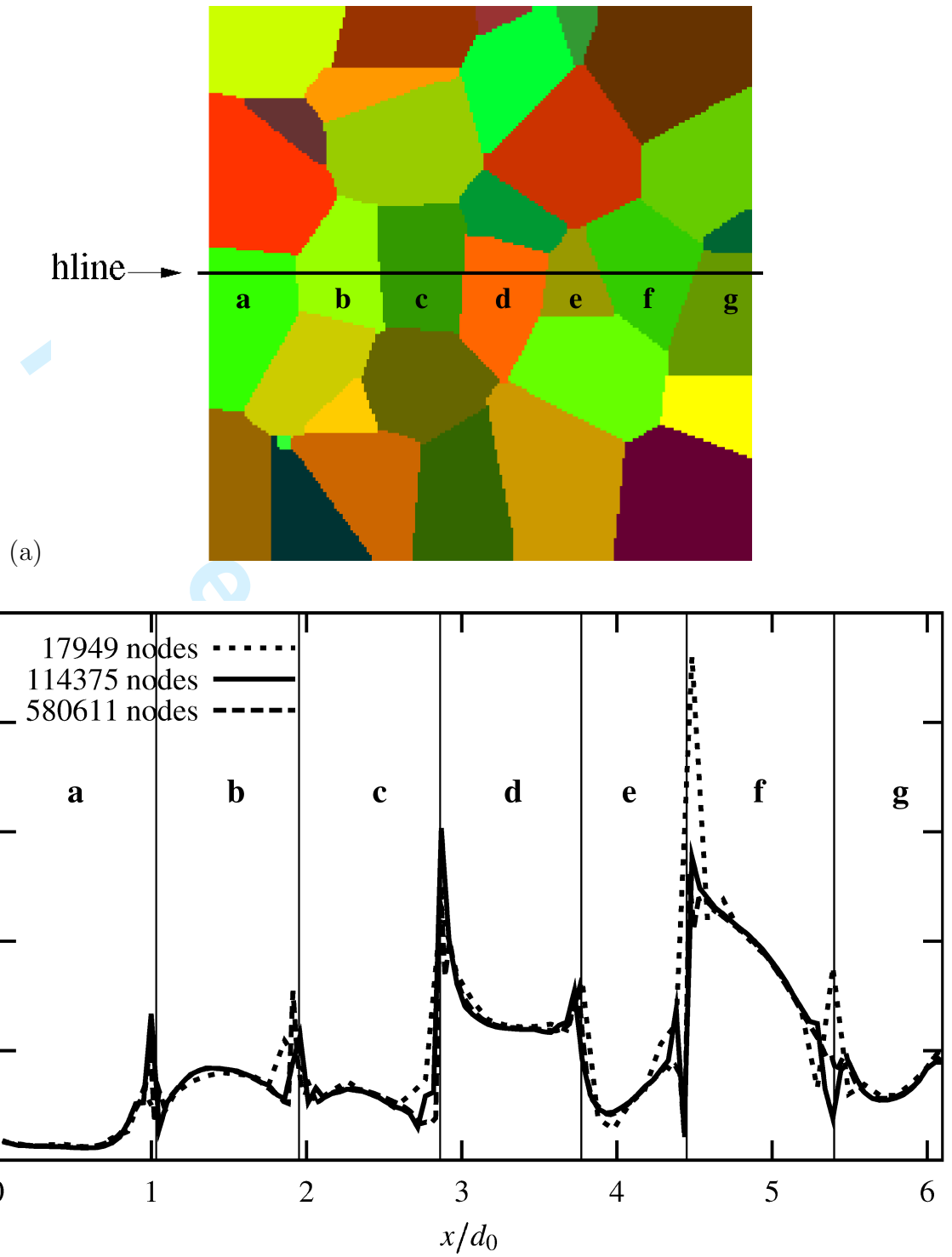
Fig. 8. Influence of mesh size on the local stress values: (a) constrained free surface used for the determination of the optimal mesh size; (b) von Mises stress profiles along the line hline shown in (a) as a function of the number of nodes of the mesh. In these calculations the morphology and crystal orientations are unchanged but different meshes are used. The vertical lines indicate the x -position of the intersection between grain boundaries and line hline . Labels have been attributed to the grains crossed by hline .
