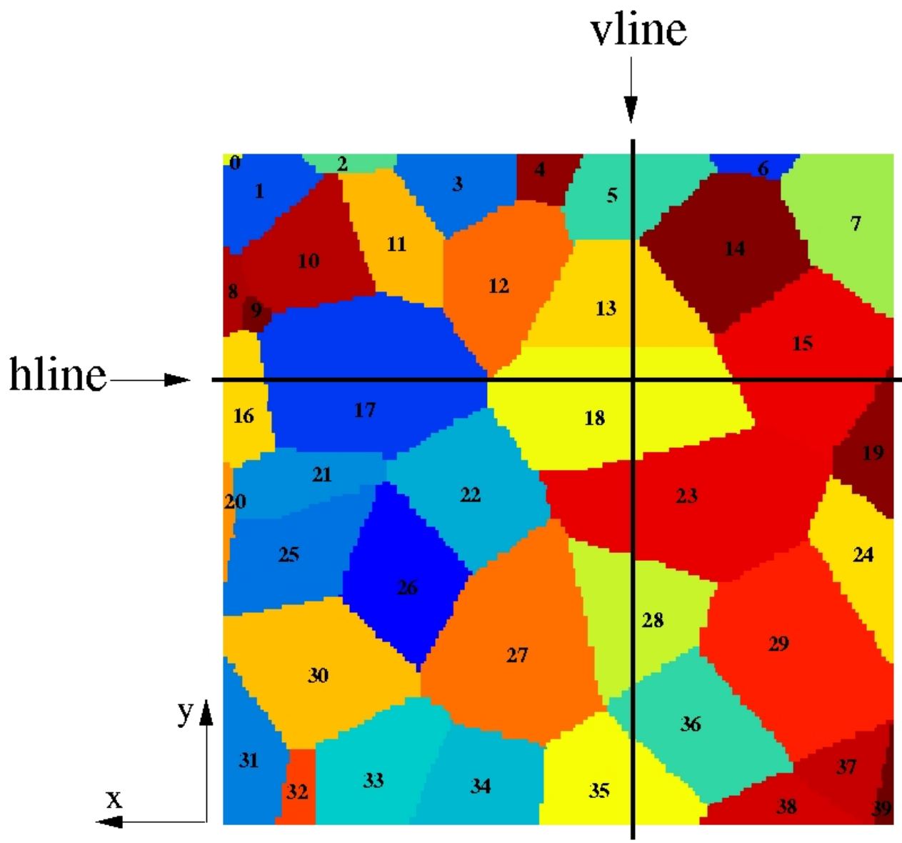
Fig. 1. Reference surface z = 0 prescribed for the construction of polycrystalline aggregates. All surface grains are labeled from 1 to 39. Two lines hline and vline have been distinguished along which mechanical variables obtained in the finite element simulations of this work have been plotted.
