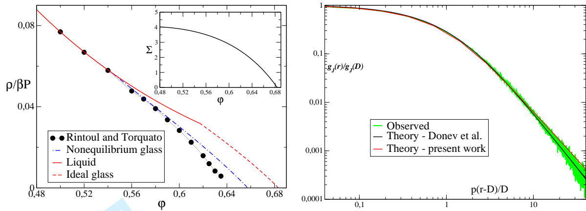
FIG. 2: (Left) Equation of state in d = 3 using the Carnahan-Starling equation of state to describe the liquid. The inverse of the reduced pressure \beta P/\rho is reported as a function of \varphi . The ideal glass transition density is \varphi_K = 0.62 and the random close packing density is \varphi_{RCP} = 0.68 . The metastable state reported in the figure correspond to a jamming density \varphi_J = 0.658 . Numerical data from [10] are reported for comparison. (Inset) Complexity as a function of the jamming density for d = 3 . (Right) Scaled correlation function g_J(r)/g_J(D) close to r = D . The theory is compared with numerical data from [14].
