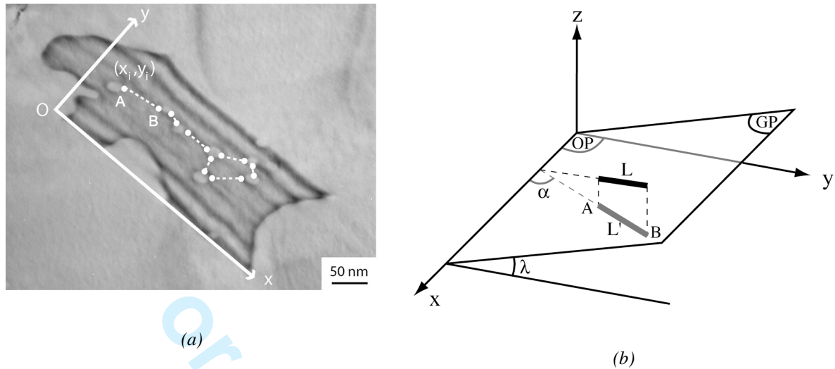
23 24 25 26 27 Figure A1. Principle of measurement of the real channel width between tertiary \gamma' precipitates in a \{111\} plane: (a) TEM image showing the apparent channels; (b) schema illustrating the corrections necessary to achieve real widths.
