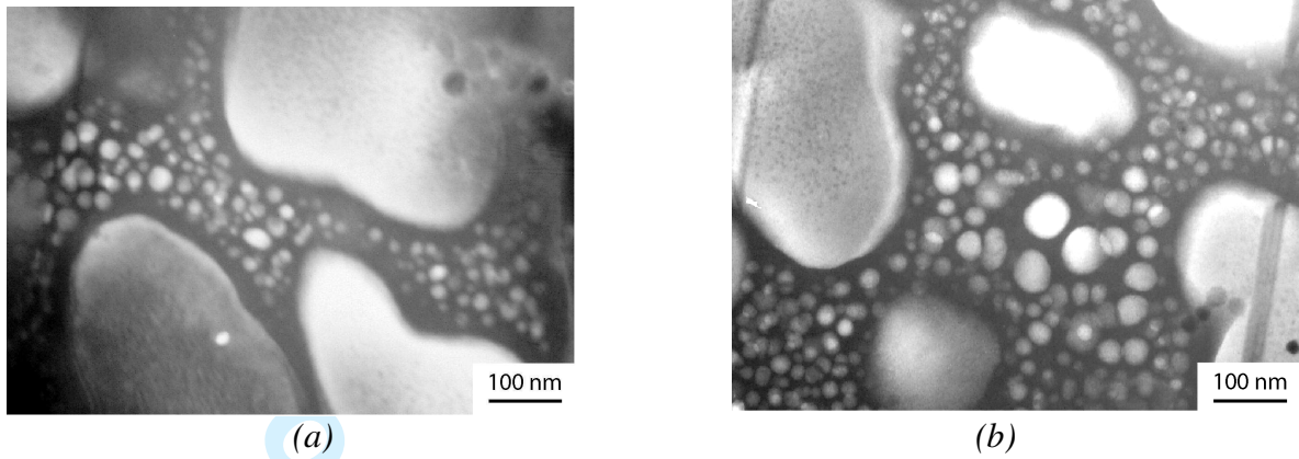
Figure 2. Dark field TEM images of the microstructure corresponding to the standard heat treatment for two different foil thicknesses a) 28 and b) 54 nm.
