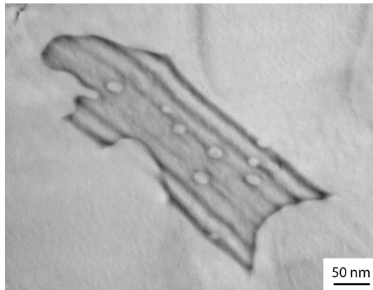
Figure 3. TEM post mortem observation in a crept sample (optimised heat treatment). Tertiary precipitates are revealed by the shearing of the matrix and by a Shockley dislocation left around them due to the shearing process described in [14].
