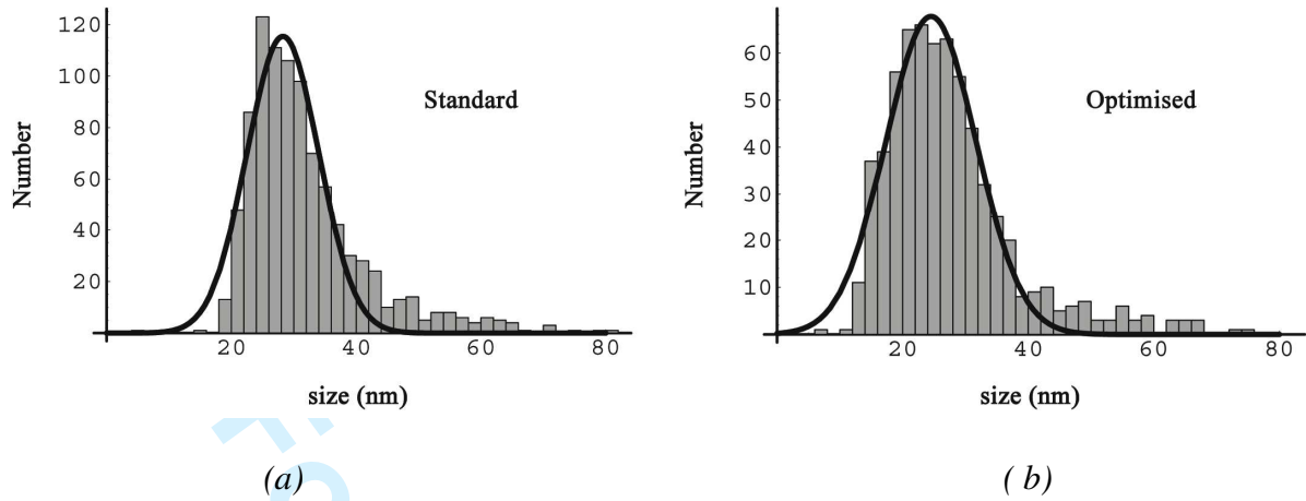
Figure 4. Diameter distribution of the tertiary precipitates produced during the (a) standard and (b) optimised heat treatments.
