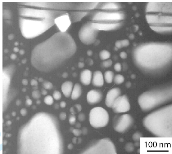
Figure 7. Dark field TEM image of the optimised microstructure. An inhomogeneous distribution of the tertiary precipitates is clearly evidenced.
