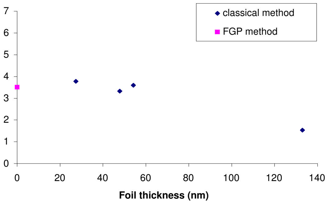
Figure 5: Influence of the foil thickness on the determination of the volume fraction using a classical method. Comparison with the FGP method. This data have been obtained for the optimised heat treatment.
