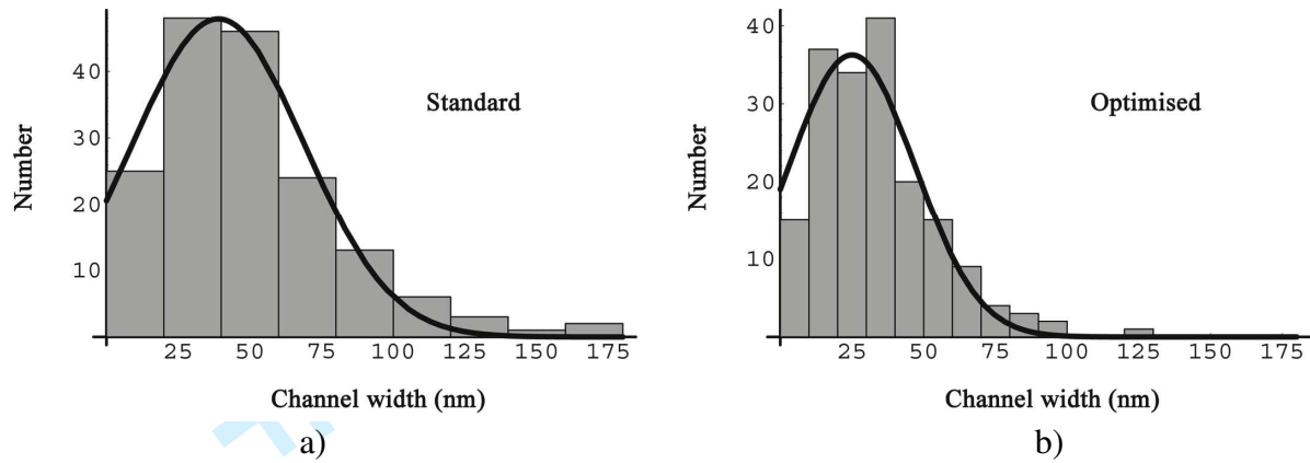
Figure 6: Channel width distributions for a) the standard heat treatment and b) the optimised one. The determinations are made using the FGP method. The estimated most probable values for channel widths are 39 nm and 25 nm, respectively.
