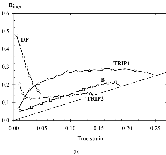
46 47 48 49 50 Figure 2 : True stress – true strain curves (a) and incremental work hardening curves (b) of the four investigated specimens.
