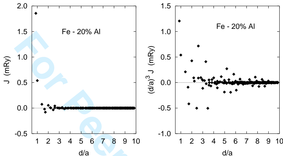
Figure 7: Exchange interactions \bar{J}_{\mathbf{R}\mathbf{R}'}^{\text{FeFe}} for a random bcc \text{Fe}_{0.8}\text{Al}_{0.2} alloy as a function of the distance |\mathbf{R} - \mathbf{R}'| = d without (left panel) and with (right panel) a prefactor d^3 .
