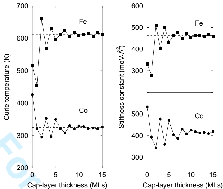
Figure 14: The Curie temperatures (left panel) and the spin-stiffness constants (right panel) of the Fe- and Co-monolayers on fcc Cu(001) as a function of the cap-layer thickness. The dashed lines represent the embedded layer limit (infinite cap thickness) while the limit of zero cap thickness corresponds to the uncovered overlayer case.
