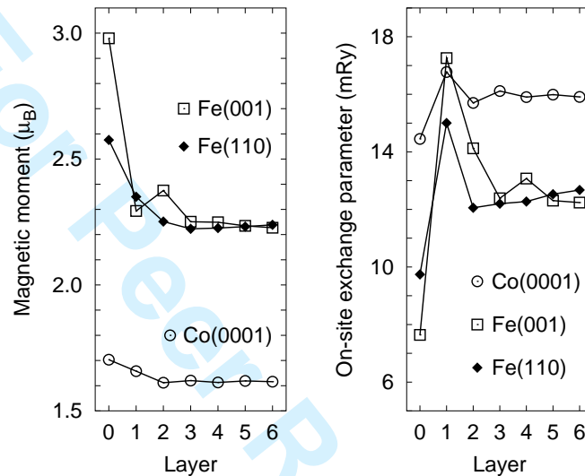
Figure 15: Layer-resolved magnetic moments (left panel) and on-site exchange parameters J_{\mathbf{R}}^0 (right panel) at surfaces of bcc Fe and hcp Co. The layer numbering starts from the top surface layer, denoted by 0.
