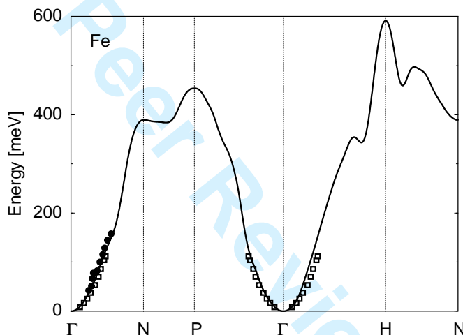
Figure 2: Magnon dispersion law along high-symmetry lines in the Brillouin zone of bcc Fe (fill line) compared to experiment (filled circles: pure Fe at 10 K [73], empty squares: Fe(12% Si) at room temperature [74]).
