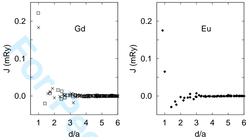
Figure 3: Exchange interactions J_{\mathbf{R}\mathbf{R}'} for hcp Gd (left panel) and bcc Eu (right panel) as functions of the distance |\mathbf{R} - \mathbf{R}'| = d . The crosses and squares in the left panel refer to pairs of sites \mathbf{R} , \mathbf{R}' lying in even (AA) and odd (AB) hcp(0001) planes, respectively.
