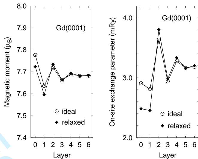
Figure 16: Layer-resolved magnetic moments (left panel) and on-site exchange parameters J_{\mathbf{R}}^0 (right panel) at the (0001) surface of hcp Gd as calculated with the lattice sites in the ideal truncated bulk positions and with the top surface layer relaxed towards the bulk. The layer numbering starts from the top surface layer, denoted by 0.
