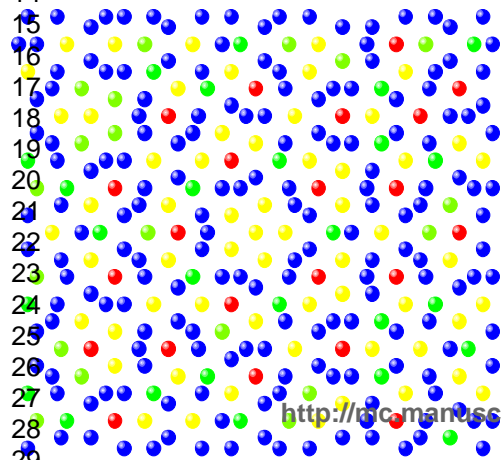
Penrose
