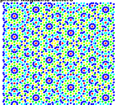
Anti - Penrose
