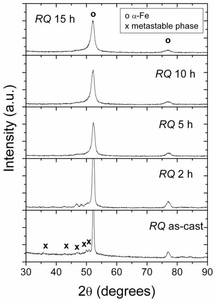
XRD patterns of powder obtained from a melt-spun ribbon after milling for different times. 205x292mm (593 x 593 DPI)
