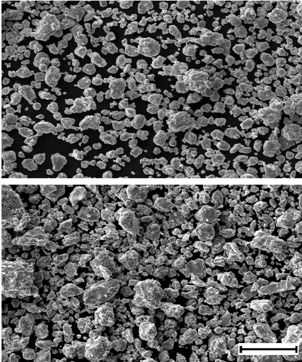
Secondary electrons SEM images of AM sample milled for 50 h (upper) and RQ sample milled for 10 h (lower). The bar corresponds to 100 \mu\text{m} .
