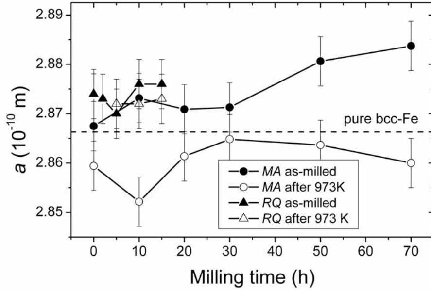
Lattice parameter, a , as a function of the milling time for both RQ and AM samples in the as-milled and annealed state. 295x203mm (593 x 593 DPI)
