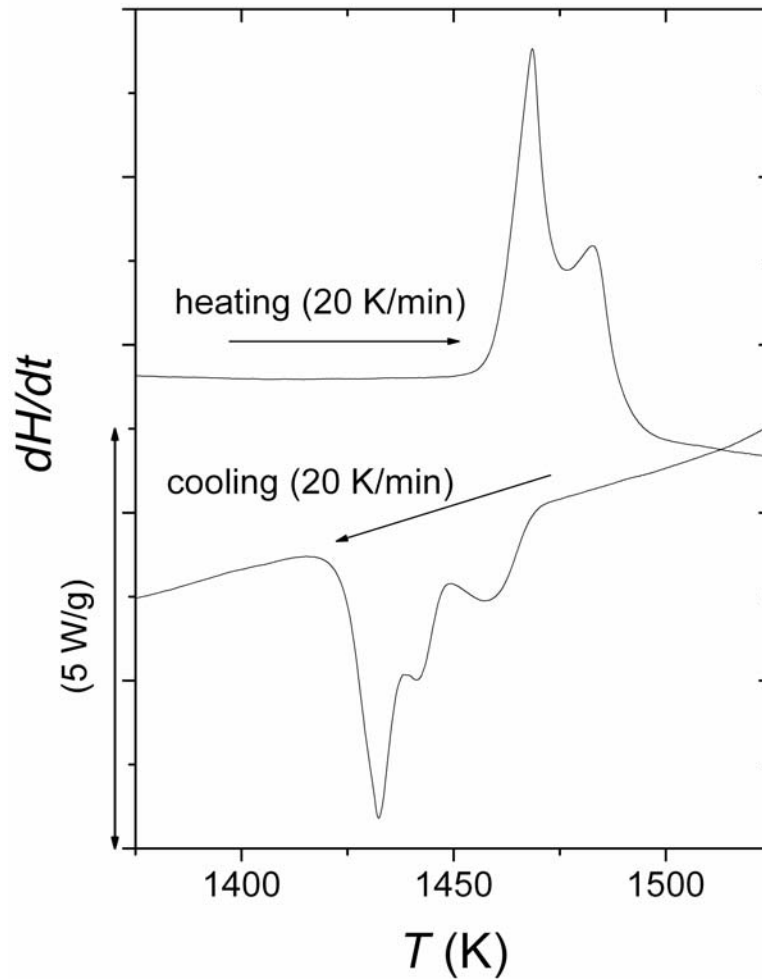
DSC scans at 20 K/min showing the melting and solidifying behaviour of the composition \text{Fe}_{78}\text{Co}_5\text{Nb}_3\text{Zr}_3\text{B}_5\text{Ge}_5\text{Cu}_1 . 203x287mm (593 x 593 DPI)
