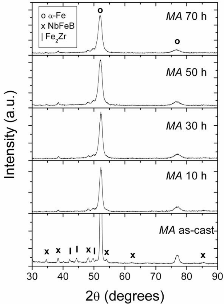
XRD patterns of powder obtained from an arc-melted alloy after milling for different times. 205x292mm (593 x 593 DPI)
