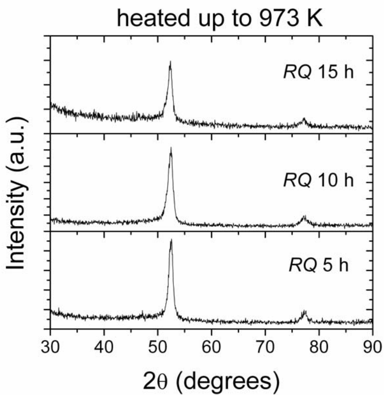
Room temperature XRD patterns of RQ samples annealed at 973 K. 205x292mm (593 x 593 DPI)
