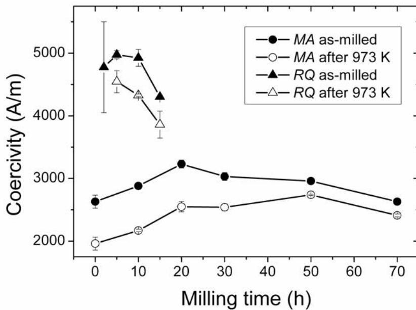
Coercivity, H_c , as a function of the milling time for both RQ and AM samples in the as-milled and annealed state.
