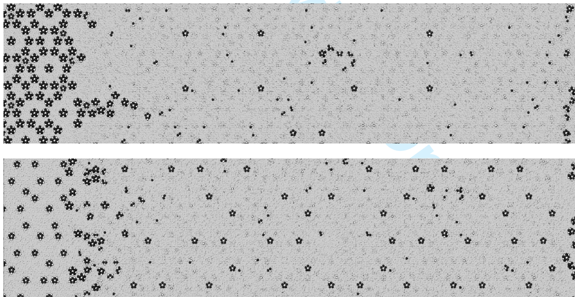
56 57 58 59 60 FIG. 9: Clusters cut by the fracture surfaces. The visualisation technique is described in Sec. III C and Fig. 6. Load: k = 1.3 , orientation: 5_2 .
