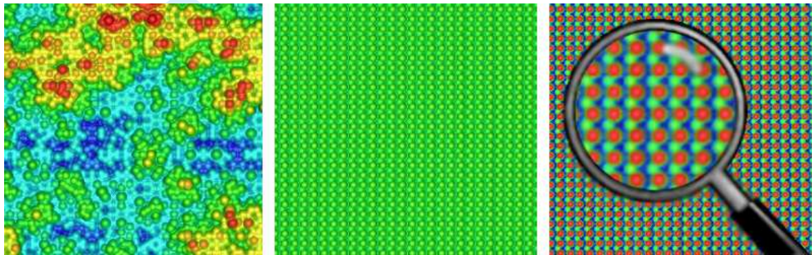
31 Figure 1: (Colour online) Sections of typical fracture surfaces of an icosahedral model qua- 32 sicrystal (left) and of a C15 model Laves phase (middle, right). The colour coding in the left 33 and middle picture is adjusted to the cluster diameter (online: from blue to red). For details 34 see text. The side length of the squares is about 14 nm. 35 36
