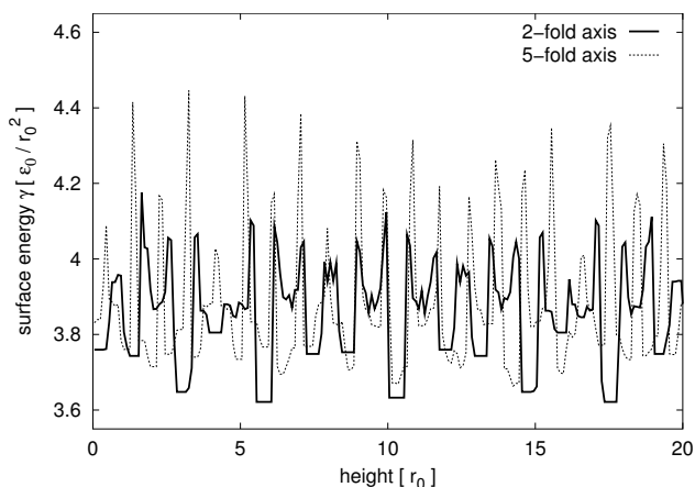
FIG. 2: Surface energy of cleavage planes perpendicular to two- and fivefold axes.
