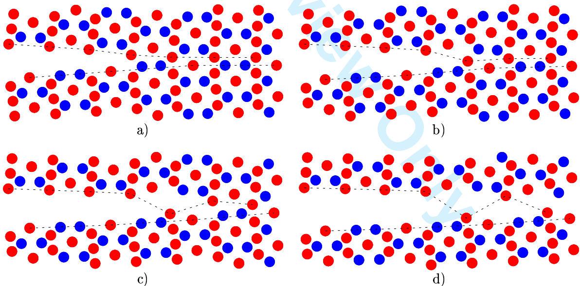
55 56 57 58 59 60 Figure 4: (Colour online) Fracture of a C15 model Laves phase: Atomic configurations in the vicinity of a propagating crack (time sequence). The fracture surface is located perpendicular to the [011] direction, the crack propagates along the [100] direction (from left to right).
