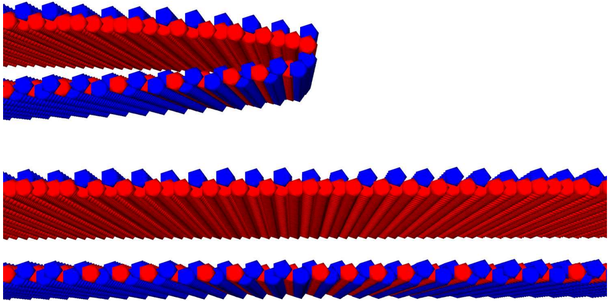
28 29 30 31 32 33 34 Figure 3: (Colour online) View inside a crack of the C15 model Laves phase. Perfect brittle cleavage fracture is observed.
