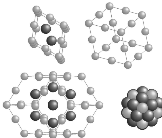
FIG. 1: Tiles of the icosahedral binary model decorated with two types of atoms and the Bergman-type cluster. Top : prolate rhombohedron (left) and oblate rhombohedron (right). Bottom : rhombic dodecahedron (left) and the 45 atoms building the Bergman-type cluster (right) inherent in the model quasicrystal. Small grey and large black spheres denote A and B atoms respectively.
