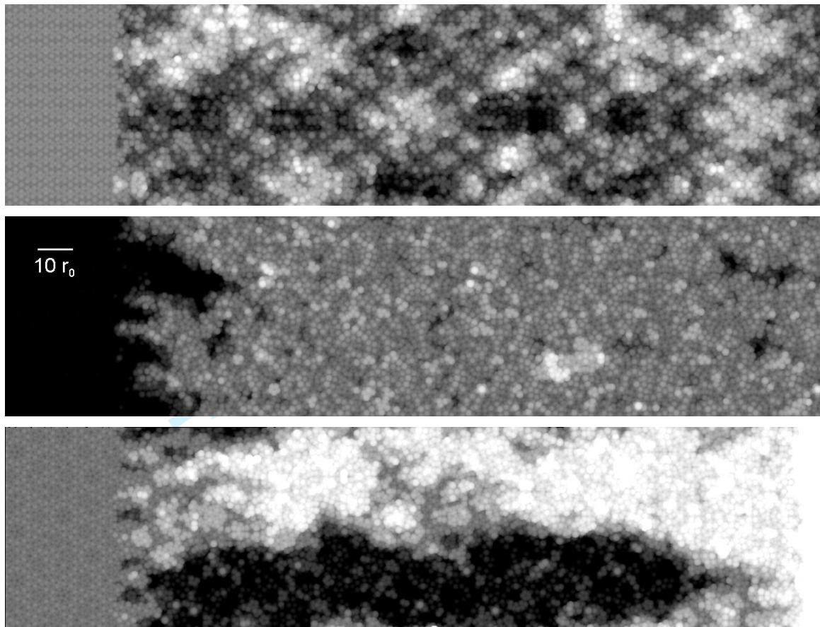
31 32 33 34 35 FIG. 8: Height profiles of sections of the simulated fracture surfaces. Load: k = 1.3 , orientation 2_2 (top), 5_2 (middle), 5_{p2} (bottom). The height increases from black ( \leq -2r_0 ) to white ( \geq +2r_0 ). The scanning sphere has the same size as an atom of type B.
