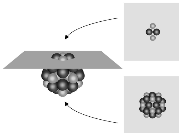
FIG. 5: Bergman-type cluster cut by a flat surface.
