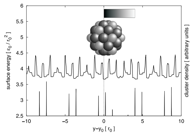
FIG. 11: Surface energy and density of cluster centres for the orientation 5_2 . The corresponding fracture surface is shown in Fig. 8, middle.
