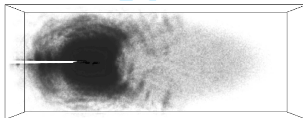
FIG. 3: Kinetic energy density. Sound waves emitted by the propagating crack and the elliptical region without damping are clearly visible. See online movie 35 .
