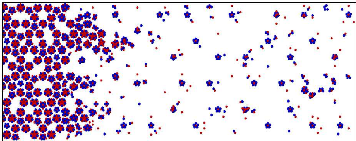
53 54 Figure 2: (Colour online) Clusters cut by the crack in a model quasicrystal: Only the smaller 55 parts of those clusters are displayed that were divided by the crack. Obviously, the dynamic 56 crack (right) intersects less clusters than the low energy seed crack (left). The cleavage plane 57 is located perpendicular to a fivefold axis, the crack propagated in twofold direction. 58 59 60
