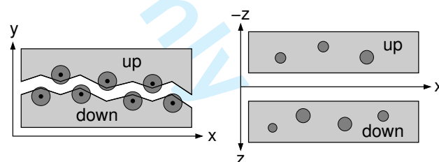
FIG. 6: Visualisation of the clusters cut by the dynamic crack. Midpoints of clusters are indicated as black dots, the clusters are idealised as spheres. The crack propagated from the left to the right. The upper and lower fracture surfaces are projected onto an x - z plane.
