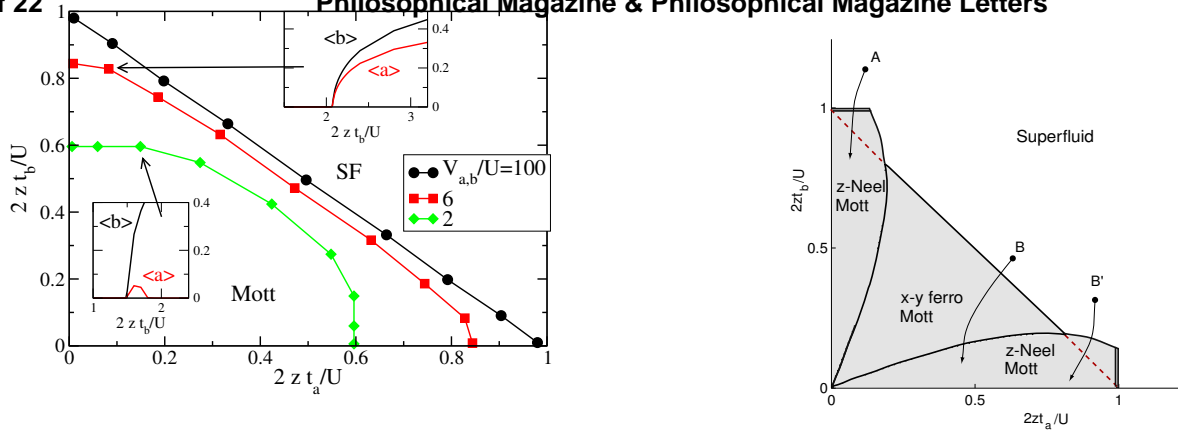
FIG. 4: Left: Phase diagram of the 2-component bosonic Hubbard model obtained via decoupling mean-field theory. Note that as V_{a(b)} decreases, the Mott domain shrinks. Right: Phase diagram including quantum fluctuations. Figures taken from (Altman et al. 2003).
