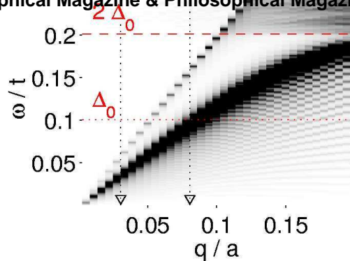
FIG. 7: Density response spectrum \chi^\rho(q, \omega) of the 2d fermionic SU(3) Hubbard model at T = 0.01t , U = -4t and filling n \approx 0.55 . Figure taken from (Honerkamp and Hofstetter 2004b).
