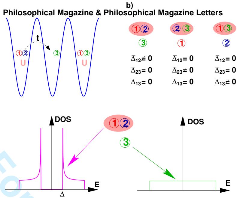
FIG. 6: BCS pairing of 3-flavor fermions with SU(3) symmetry. Note that one flavor remains unpaired, with a normal Fermi surface. Figures taken from (Honerkamp and Hofstetter 2004b).
