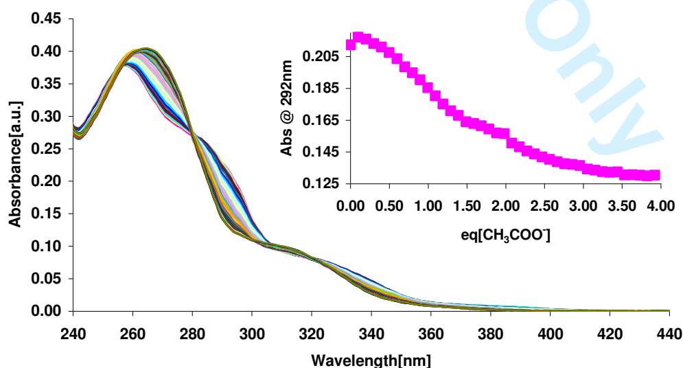
Figure 3. Changes on the absorbance of 1 3 Eu (4 \mu M) upon addition of AcO - . Insert: shows changes in absorbance at 292 nm as a function of equivalents of acetate added.
