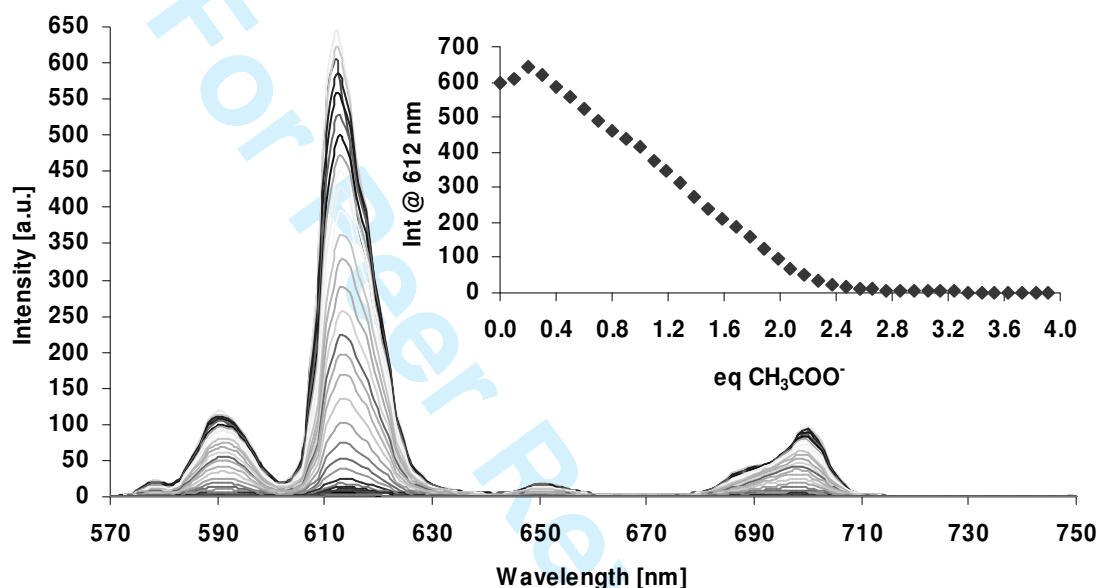
Figure 4. Changes on the lanthanide emission intensity of 1 3 Eu (4 \mu\text{M} ), which was quenched upon titration with \text{AcO}^- . Insert shows changes in intensity at 612 nm as a function of added equivalents of \text{AcO}^- .
