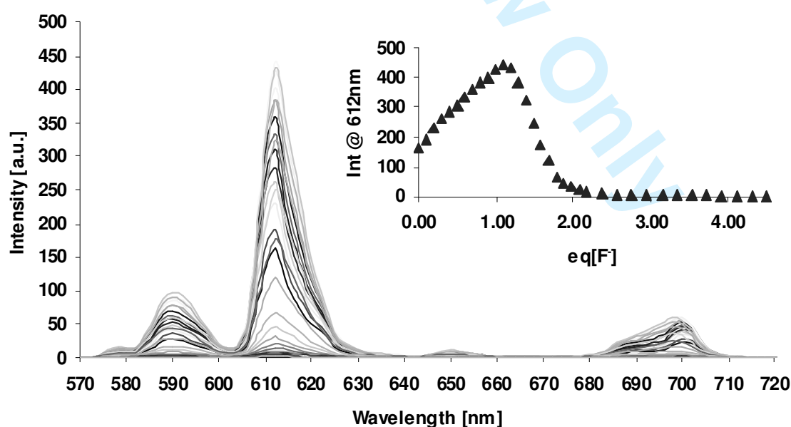
Figure 5. The overall changes on the Eu(III) emission of \text{Eu}^{3+} (4 \mu\text{M} ) upon addition of \text{F}^- . Insert: The changes in the intensity at 612 nm as a function of added equivalents of \text{F}^- .
