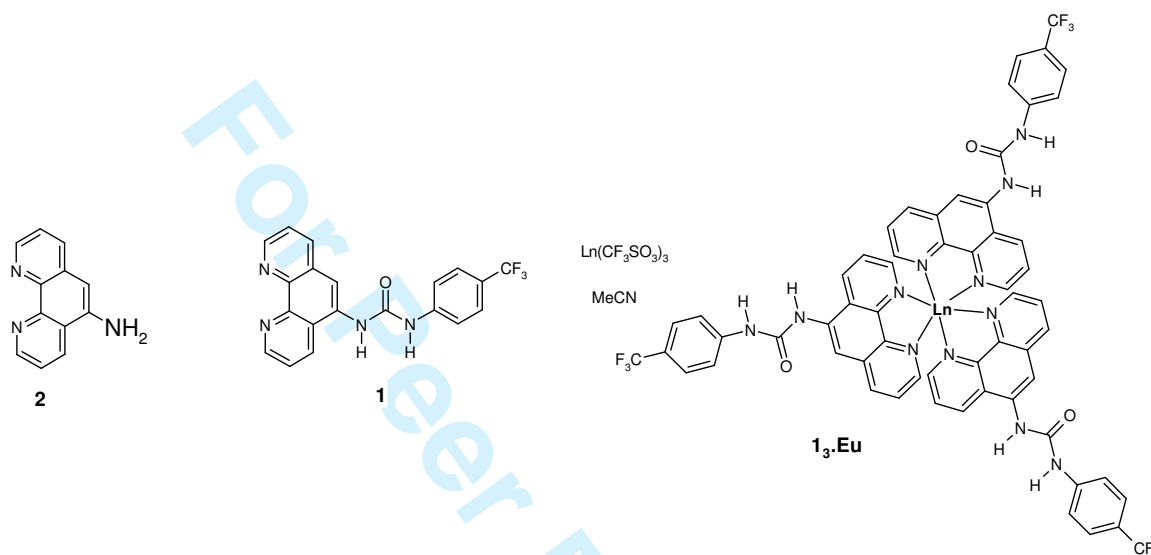
Scheme 1. Synthesis of 1 and the Eu(III) complex of 1 , 1 3 Eu (several structural isomers were expected to be formed).
