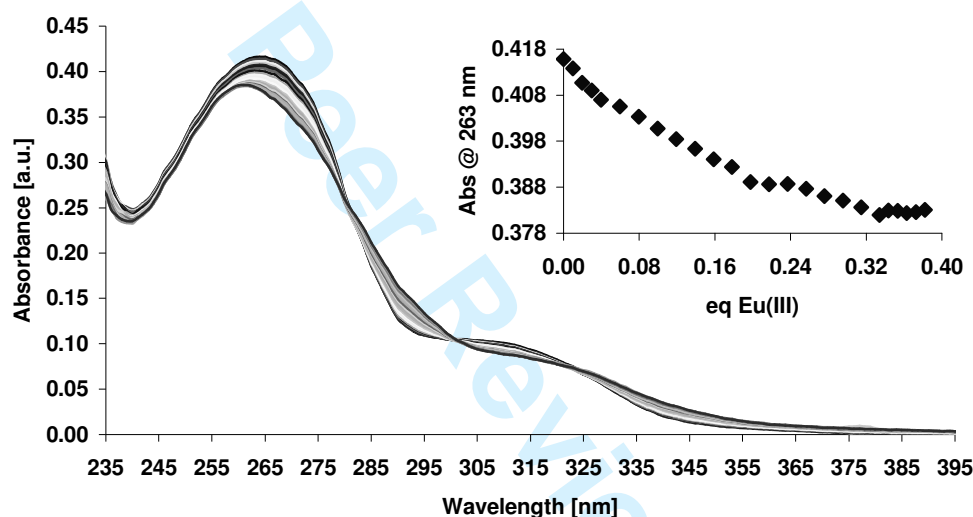
Figure 1. Changes on the absorption spectra of 1 (10 \mu\text{M} ) upon addition of \text{Eu}(\text{CF}_3\text{SO}_3)_3 . Insert: The changes in absorbance at 263 nm as a function of equivalents of \text{Eu(III)} .
