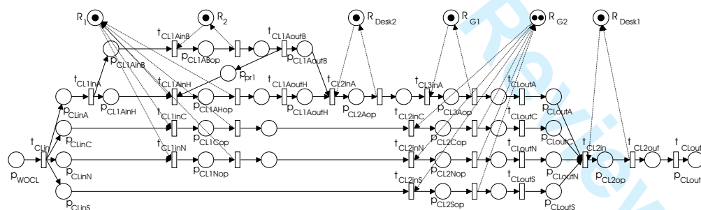
Figure 15. PN model of product 'Corner clamp L'.
