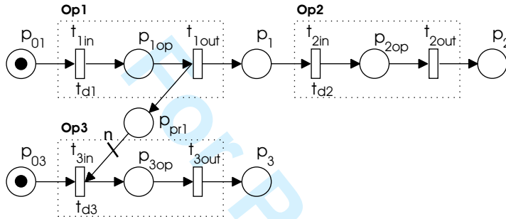
Figure 6. Precedence constraint.
