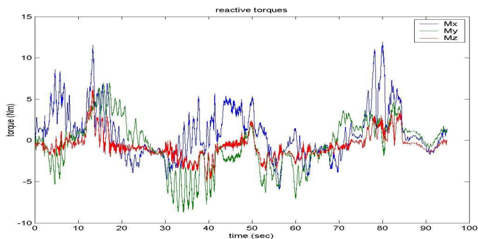
figure 3 : Reactive torques using hard brush at 700 rpm
