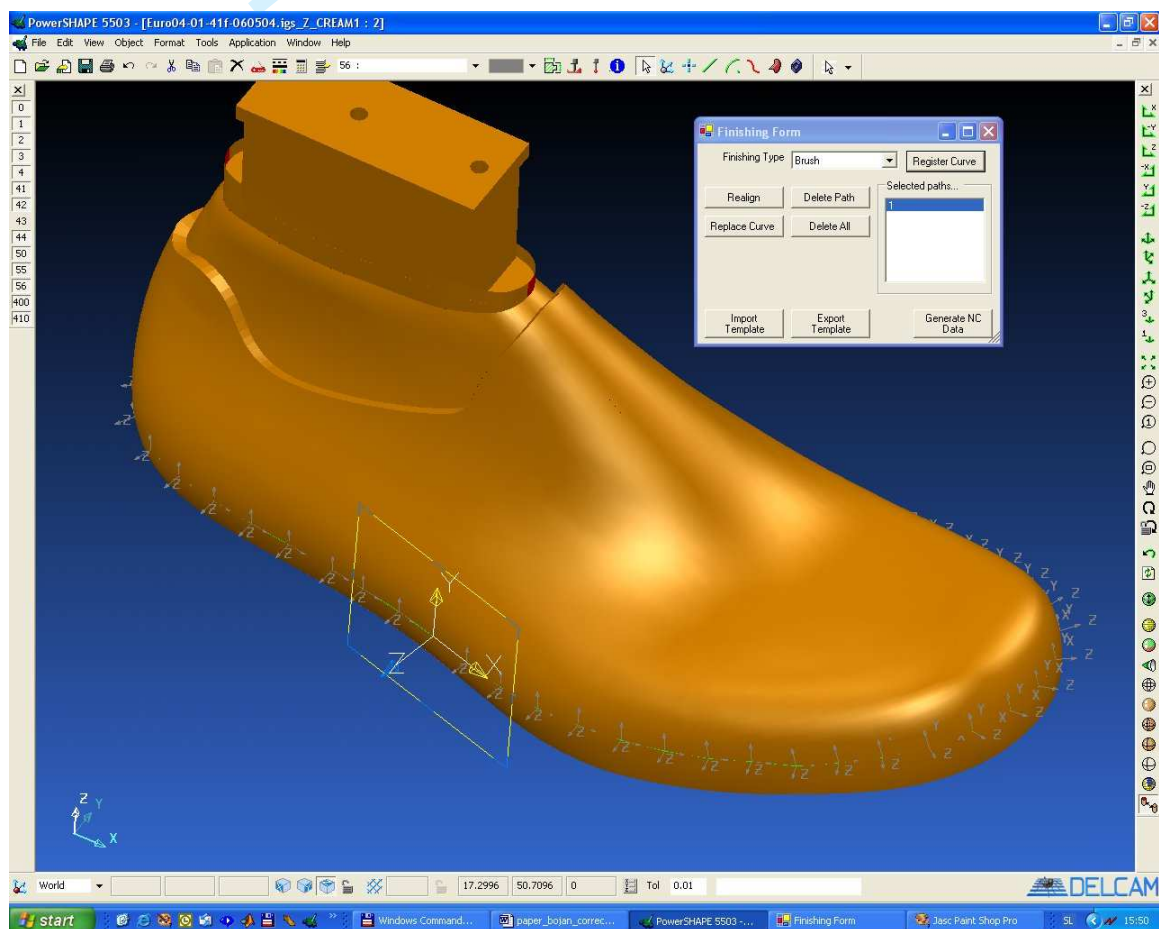
figure 8 : Trajectory generation with PowerShape CAD program
