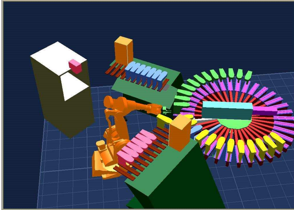
figure 5: Display of the simulated cell on ROBCAD
