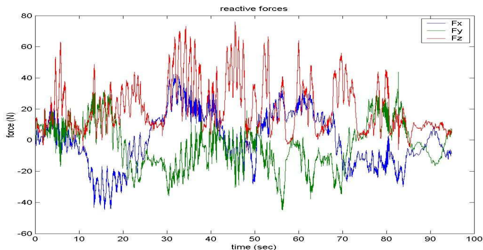
figure 2 : Reactive forces using hard brush at 700 rpm
