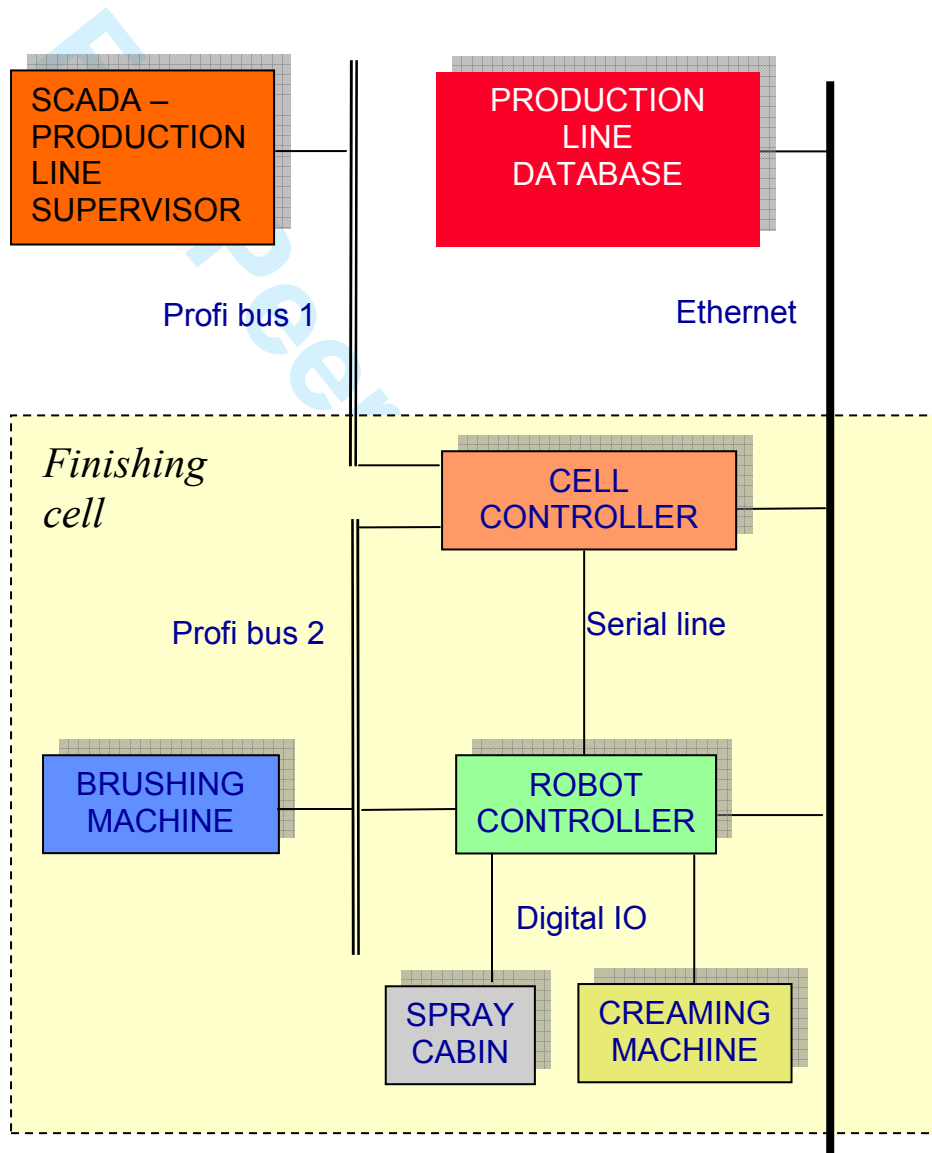
figure 7 : Block diagram of the finishing cell control
