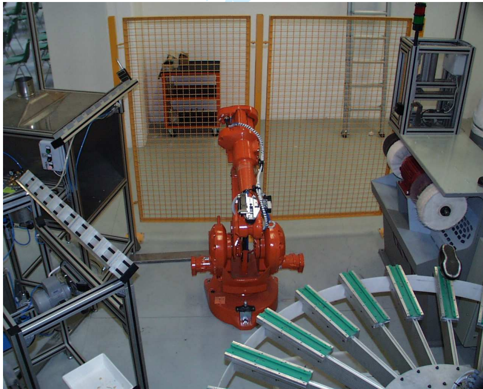
figure 6: Actual finishing cell
