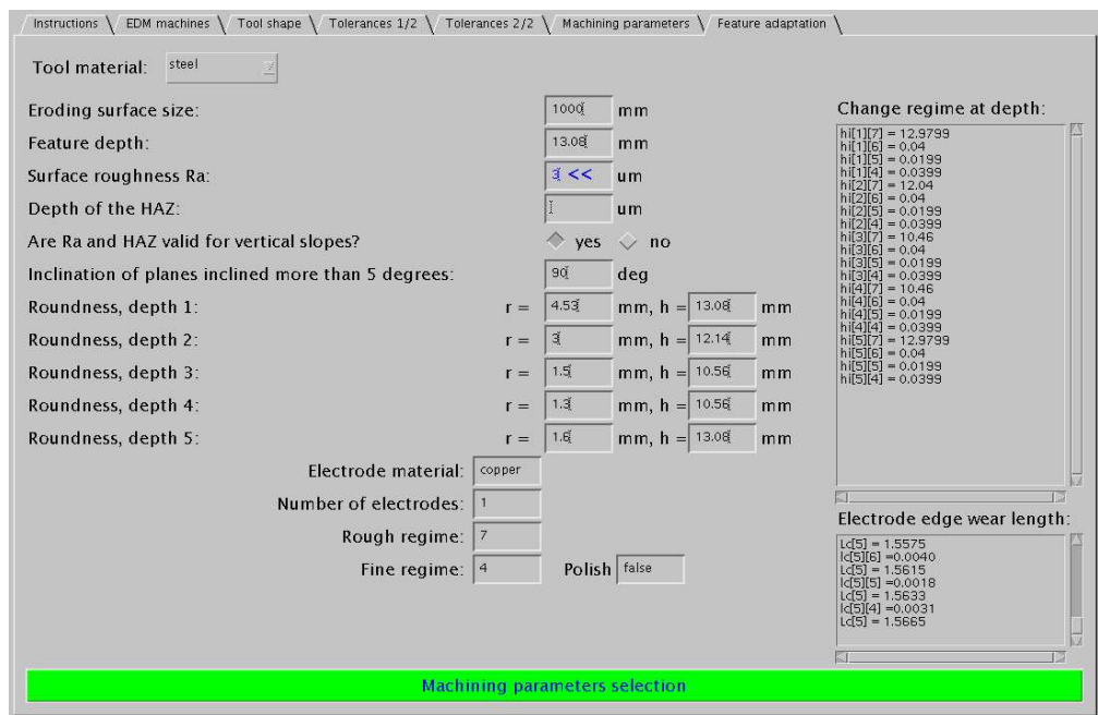
Feature adaptation for the ease of manufacturing - design and manufacturing parameters after the adaptation. 386x251mm (72 x 72 DPI)
