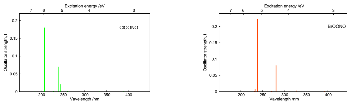
Figure 3. Calculated electronic spectra of ClONO and BrONO.
