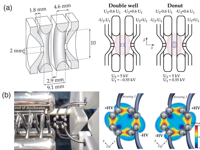
FIG. 9: Electric trapping of polar molecules. (a) Electrostatic trap for confining low-field seeking molecules in various trapping geometries. (b) Linear AC trap for high-field and low-field molecules, showing the two electric field configurations used for electrodynamic trapping. Adapted from Refs. [78, 179].
