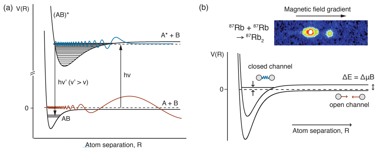
FIG. 6: (a) Photoassociation of laser-cooled atoms. Illumination of an ultracold atomic gas with a laser tuned to slightly below the atomic excitation frequency allows a pair of colliding atoms to absorb a photon. This absorption forms a vibronically excited dimer state which can then decay either by stimulated or spontaneous emission to bound states of the ground electronic potential. (b) Feshbach resonance magnetic tuning. The energy difference of two potential energy curves which correlate with different hyperfine states of the colliding atoms can be tuned using external magnetic fields. At certain field strength the colliding atoms are converted to molecules. The inset shows an absorption image of two Rb atomic clouds produced by separating and then dissociating the molecules (right) from the original atom cloud (left). Experimental results adapted from Ref. [143].
