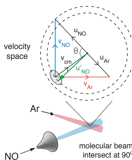
FIG. 8: Newton diagram for single collision cooling. Molecular beams of NO and Ar intersect at right angles and scatter over a wide range of angles. A small fraction of NO ( ^2\Pi_{1/2} , j = 1/2 ) molecules are inelastically scattered through angles close to \theta , into the ^2\Pi_{1/2} , j' = 15/2 rotational state. For these molecules, the centre-of-mass frame velocity cancels the laboratory frame velocity, producing a stationary distribution (shaded area). The dashed circles represent the limiting the centre-of-mass recoil velocities for elastically scattered (outer) and inelastically scattered (inner) NO molecules.
