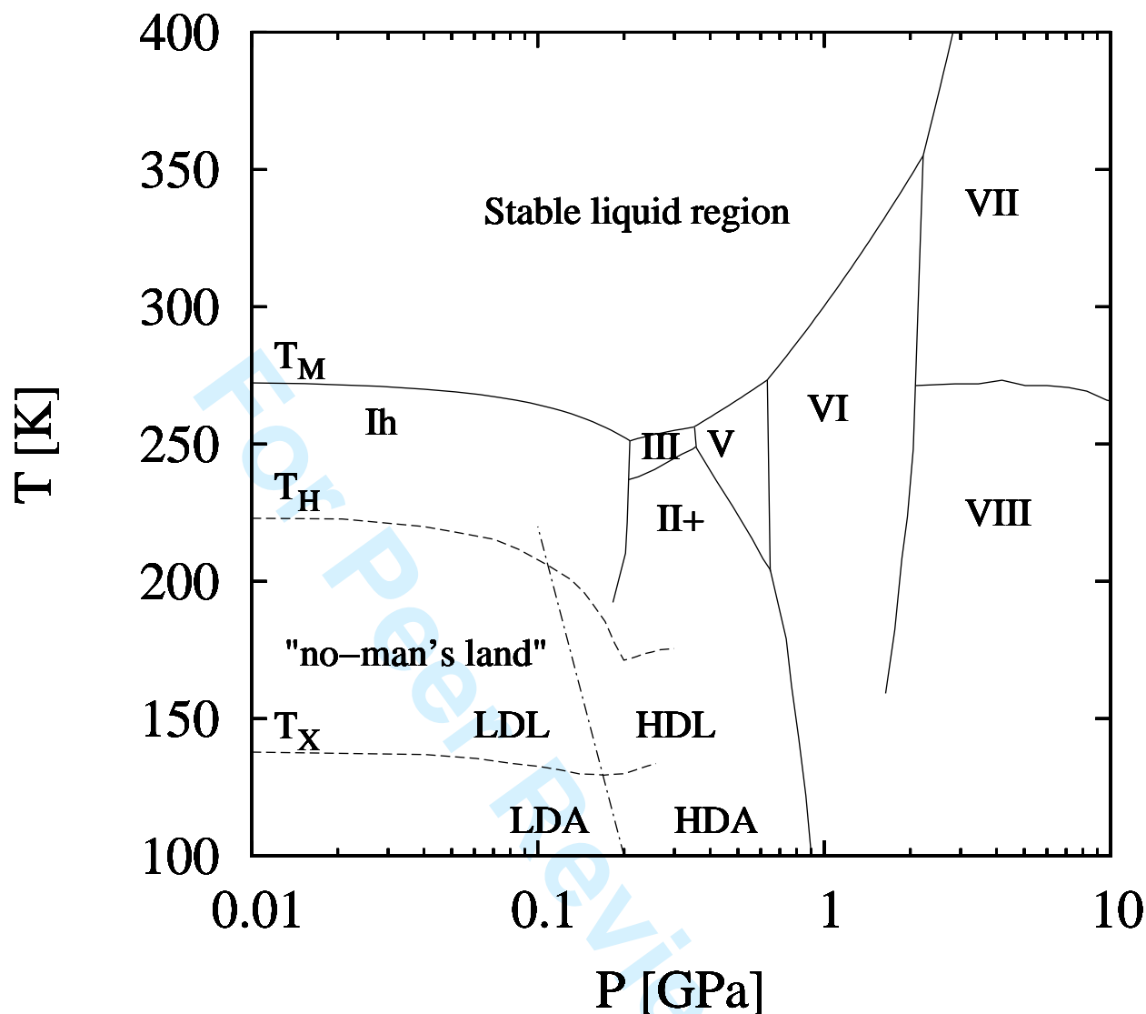
FIG. 1: The temperature-pressure phase diagram of water showing the melting line, T_M (solid), the homogeneous nucleation line, T_H (dashed), and the crystallisation line, T_X (dashed), which represents the highest temperature that amorphous ice can exist without crystallisation. The region between T_X and T_H is called "no-man's land". The liquid-ice melting lines are taken from [6]. The homogeneous nucleation line is taken from [7]. The crystallisation line of amorphous ice is taken from [8]. The transformation lines between the different ices are sketched in approximately for completeness. The region labelled ice II+ contains more than one form of ice. Also shown is the conjectured line of LDL - HDL (or LDA - HDA) transitions based on the available data, [9–11] (dot-dashed line).
