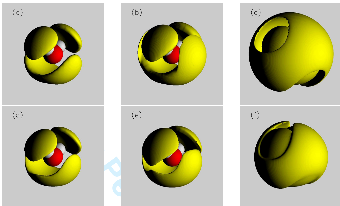
FIG. 9: Spatial density functions, g(r, \theta, \phi) , for low (top, (a) - (c)) and high (bottom, (d) - (f)) density water. These are shown over the distance ranges 0 - 3.55Å for (a) and (b), 0 - 3.09Å for (d) and (e), 0 - 4.24Å for (c), and 0 - 3.65Å for (f), corresponding to coordination numbers of 4 for (a),(b),(d), and (e), and 8 for (c) and (f). Contour levels are set to include 90% of the molecules in the distance range for (a) and (d), 100% of the molecules in the distance range for (b) and (e), and 80% of the molecules in the distance range for (c) and (f). We see that the inner shell of 4 molecules changes very little on compressing LDL to form HDL, remaining primarily tetrahedral in local coordination, but there is a marked shift inwards of the second shell with increased density, corresponding to the marked change in bond angle distribution, Fig. 8.
