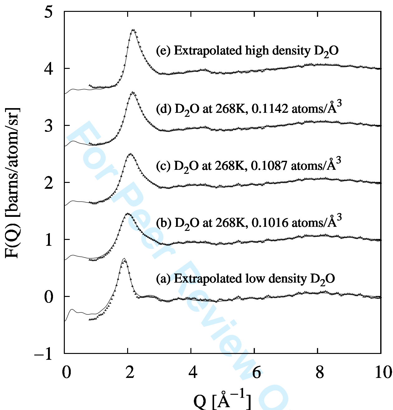
FIG. 3: The differential cross section of heavy water at 268K at three measured densities, as well as extrapolated data to low and high density. (a) is the extrapolated LDL at 0.0885 \text{ atoms}/\text{\AA}^3 , (b) - (d) are the experimental data at densities 0.1016 , 0.1087 and 0.1142 \text{ atoms}/\text{\AA}^3 respectively, and (e) is the extrapolated data to 0.1206 \text{ atoms}/\text{\AA}^3 . From [3]. The lines show the EPSR fits to these data. Note that the qualitative differences between LDL and HDL as shown in (a) and (e), linearly extrapolated from the measured data at intermediate densities, are mirrored in the data for LDA and HDA, Fig. 2. Note that the statistical quality of these data is much worse than for the amorphous ices because of the large ( \sim 95\% ) contribution to the scattering from the pressure containment cell which has to be subtracted in the data analysis.
