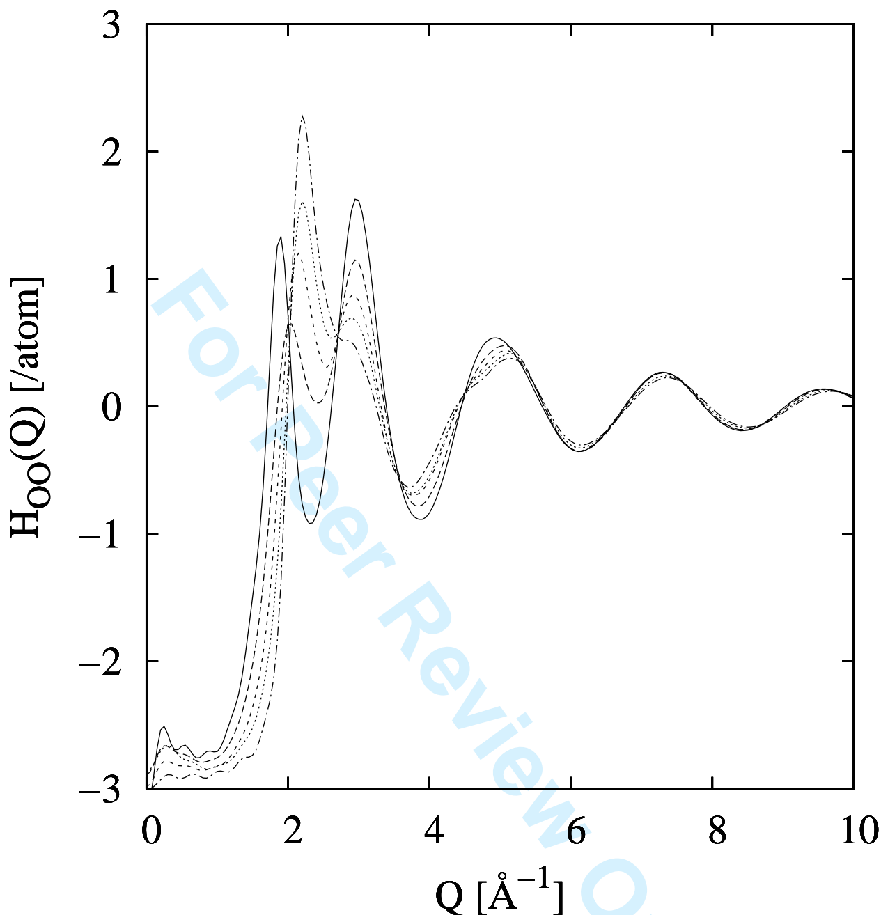
FIG. 4: The OO partial structure factors derived from the EPSR simulations shown in Fig. 3. The solid line is case (a), dashed line case (b), narrow dashed line case (c), dotted line case (d), and dot-dashed line case (e). We note that there is a marked change in the first peak positions with density, and that there are ‘isosbestic’ points - places where all the curves pass through the same value. These points arise from the linear nature of the change in the structure with density. Such points have traditionally been used to indicate that intermediate states are composed of a mixture of the two end point states, but as can be seen from the lack of low Q scattering, there is not sign of heterogeneities within the length scale of the simulations or data ( \sim 36\text{\AA} ). Hence the system remains homogeneous throughout the transition.
