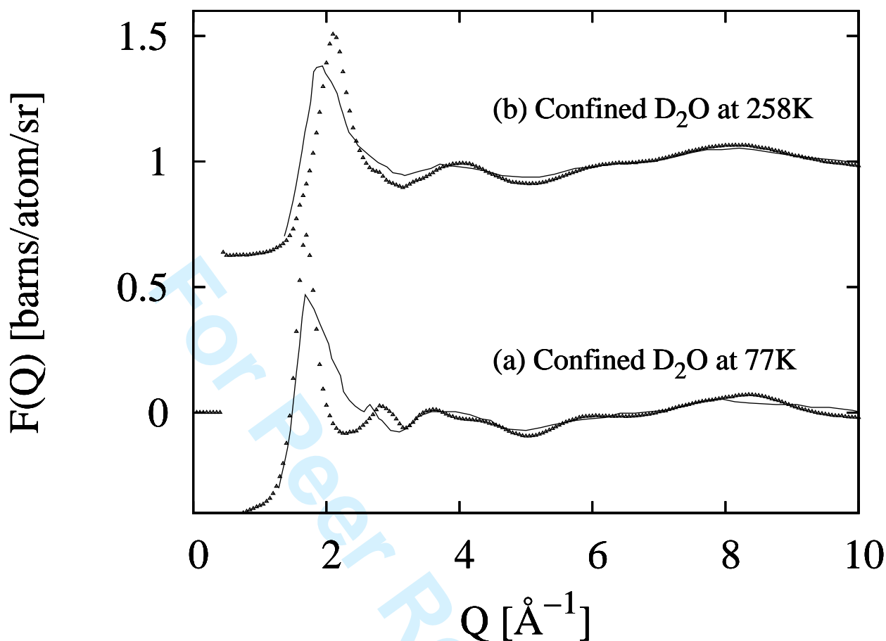
FIG. 2: The differential cross section of highly confined heavy water obtained by Zanotti et. al. at (a) 77K and (b) 258K, (lines, [67]). Also shown are the diffraction data for (a) LDA and (b) HDA (triangles, [77]). It is apparent that at 258K the first peak of the confined water does not coincide with that of HDA, and that at 77K the structure beyond the first peak in confined water does not match that seen in LDA.
