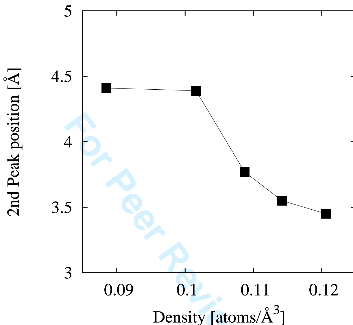
FIG. 6: Position of the second peak in the OO radial distribution functions derived from the EPSR simulations shown in Fig. 5. We see the peak position is initially constant, then changes rapidly with increasing density.
