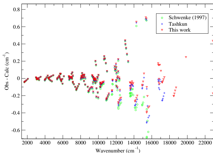
Figure 5. Comparison of calculated HDO energy levels with J = 5, p = 1 to experimental data [86–97] for this work and previous calculations [56, 84].
