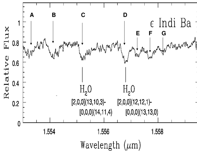
Figure 4. Spectrum of brown dwarf \epsilon Indi Ba as reported by Smith et al [55]. Features labelled \text{H}_2\text{O} were assigned in the original work; the letters refer to assignments presented in table 3.
