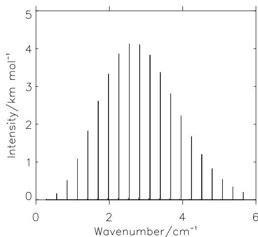
Figure 3. The rotational spectra of \text{Co}^{12}\text{CN} and \text{Co}^{13}\text{CN} with the C isotopes in their natural abundances simulated ab initio at T = 12 K.
