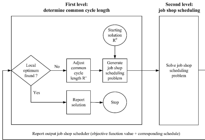
< Figure 2: Two-level procedure for solving NLP >
