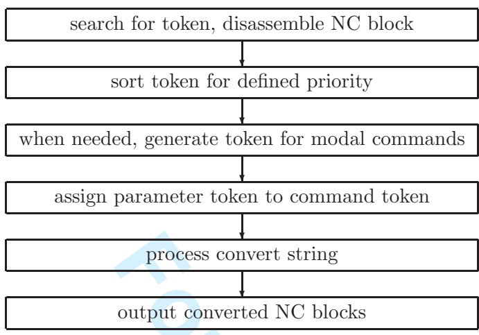
Figure 4. Structure of the conversion process
