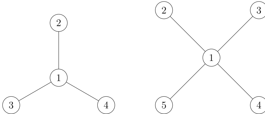
Figure 3: The star graphs S_4 and S_5 .
