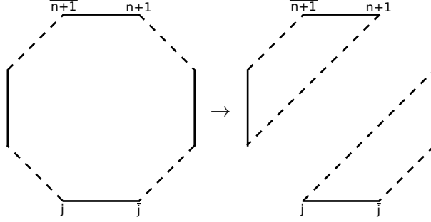
FIGURE 4. G_\sigma and G_{(n+1, j)\sigma} in the “cut” case
