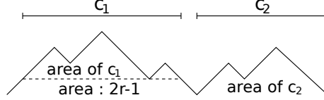
FIGURE 5. First-passage decomposition of a Dyck path
