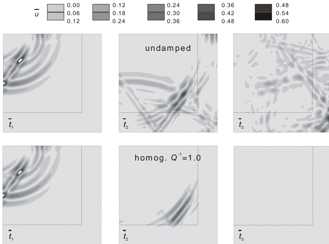
Fig. 6. Comparison between the undamped case (top) and the homogeneous case ( Q_{\min}^{-1} = 1.0 , bottom) at three different times: normalized displacement at \bar{t}_1 = t_1 / t_p = 4.15 (left) ; \bar{t}_2 = t_2 / t_p = 9.13 (centre) ; \bar{t}_3 = t_3 / t_p = 14.1 (right).
