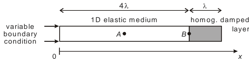
Fig. 2. Schematic of the first numerical test: undamped elastic layer (left) and homogeneously damped layer (right)
