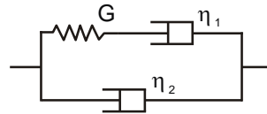
Fig. 1. Rheological model for a Generalized Maxwell fluid leading to the same damping properties as the Rayleigh formulation [33,34].
