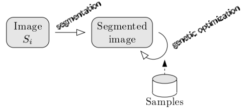
(c) optimized watershed : supervised segmentation by parameters optimization (Sec. 4)
