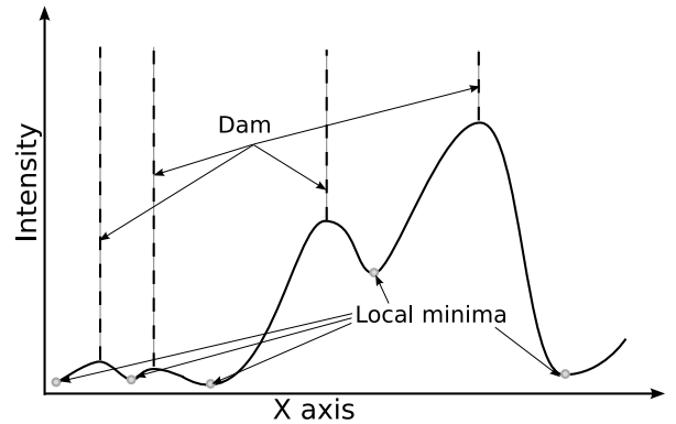
Figure 1: Illustration of the watershed segmentation principle. For each pixel, the elevation relies here on the intensity within the image.
