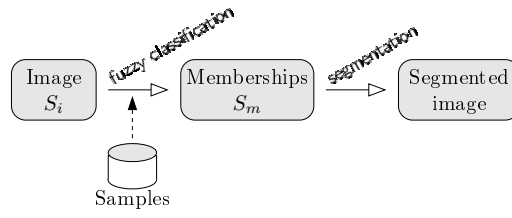
(b) probashed : supervised segmentation by space transformation (Sec. 3)
