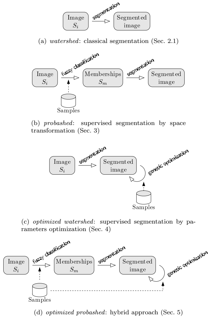
Figure 3: The different segmentation processes presented in this paper
