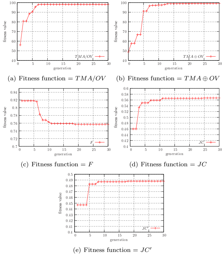
Figure 5: Evolution of the fitness functions according to the number of generations
