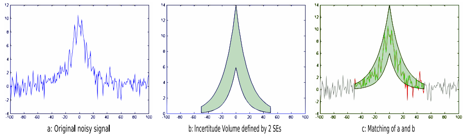
Figure 3: Example of application of the fuzzy HMT to detect an exponential profile with Gaussian noise. Image (a) represents a 1D noisy signal ( \text{SNR} \approx 9\text{dB} ). Image (b) represents the uncertainty area defined by the 2 SEs F and B . Image (c) shows how well the pattern can fit the signal.
