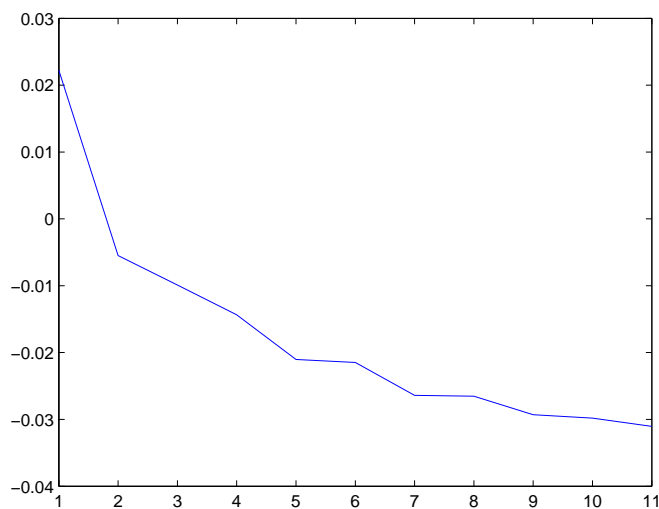
FIGURE 2. Minimizing the Motzkin-like polynomial in [0, 1]^2
