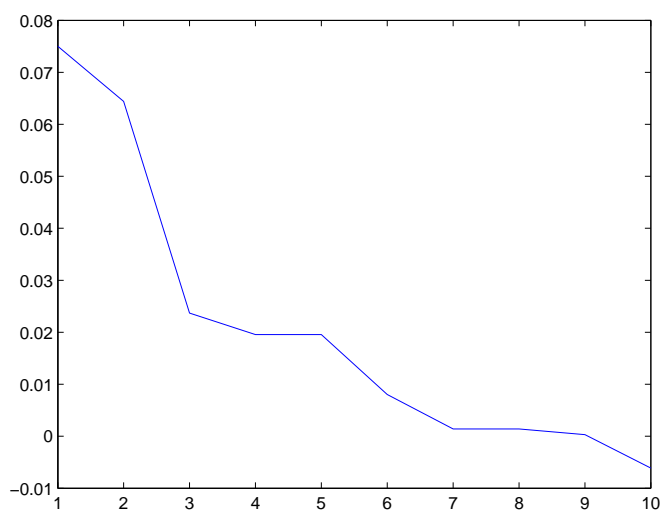
FIGURE 5. Minimizing 0.375 - 5x + 21x^2 - 32x^3 + 16x^4 on [0, 1]
