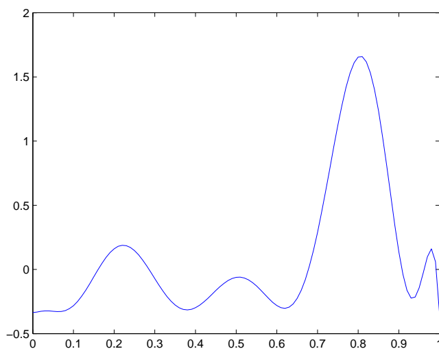
FIGURE 6. The probability density \sigma(x)dx on [0, 1]
