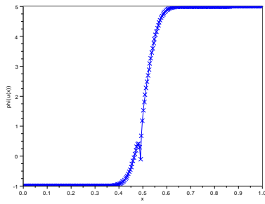
(c) \phi(u) as a function of x
