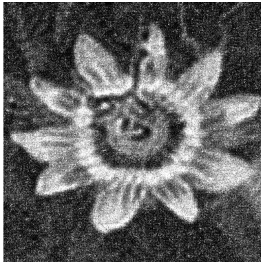
(c) Itération 10
