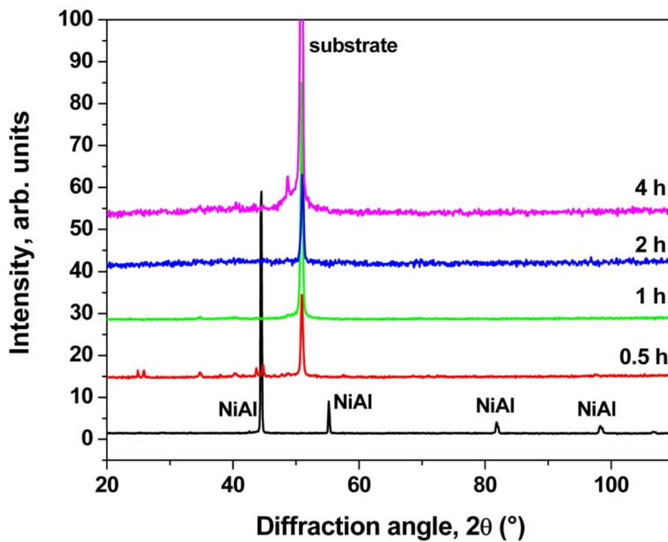
Figure 5.- XRD patterns of the aluminised superalloy samples as a function of stripping immersion time in bath A (Pitting acid- Organic media) at T=50°C.
