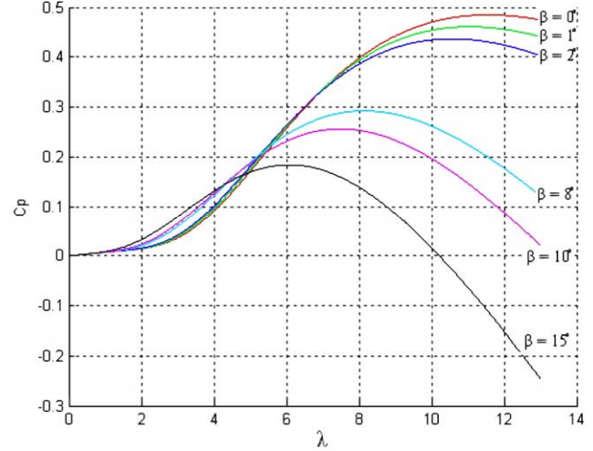
Fig 3 The power coefficient of a variable speed turbine
